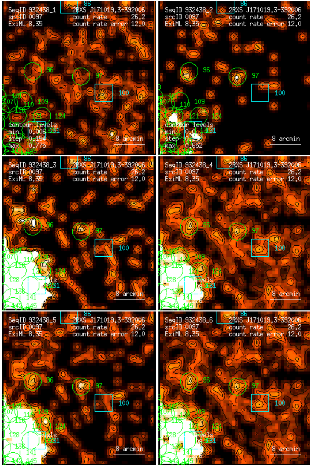
Figure 97: RASS 932438: detection 0097: band rate images, Gaussian filter: (1) PSPC channels 11 – 41, (2) 52 – 90, (3) 91 – 201, (4) 11 – 235, (5) 52 – 201, (6) 11 – 201. Broad band rates in counts/ks. Band rate contour levels in counts/ks/arcmin 2 .
