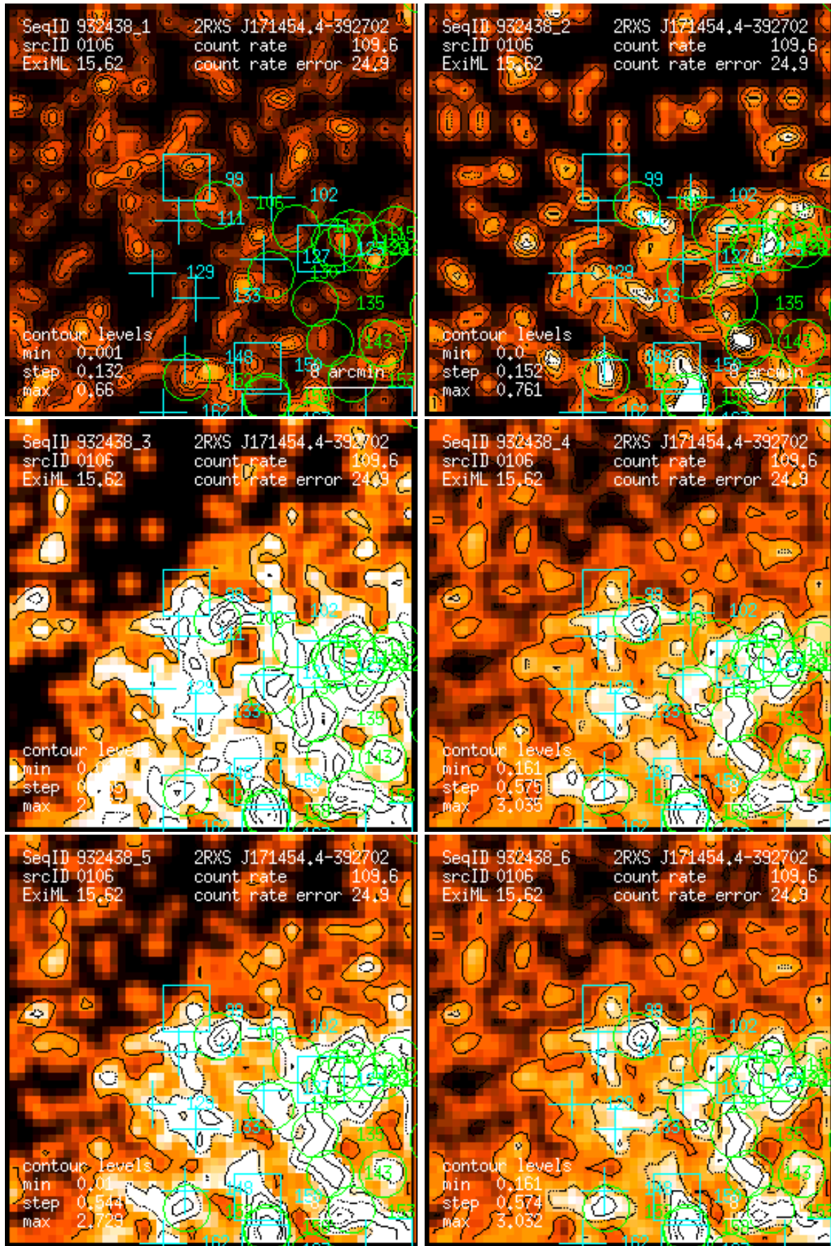
Figure 106: RASS 932438: detection 0106: band rate images, Gaussian filter: (1) PSPC channels 11 – 41, (2) 52 – 90, (3) 91 – 201, (4) 11 – 235, (5) 52 – 201, (6) 11 – 201. Broad band rates in counts/ks. Band rate contour levels in counts/ks/arcmin 2 .
