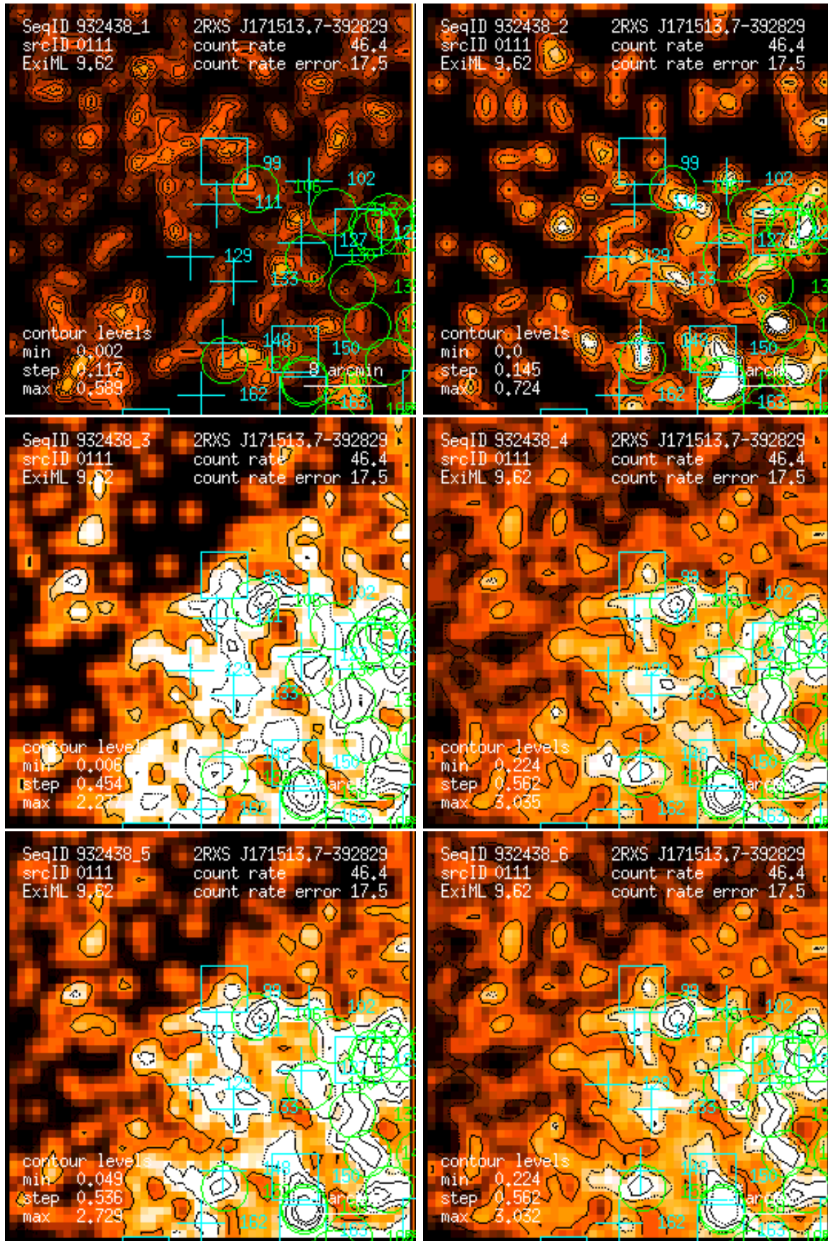
Figure 111: RASS 932438: detection 0111: band rate images, Gaussian filter: (1) PSPC channels 11 – 41, (2) 52 – 90, (3) 91 – 201, (4) 11 – 235, (5) 52 – 201, (6) 11 – 201. Broad band rates in counts/ks. Band rate contour levels in counts/ks/arcmin 2 .
