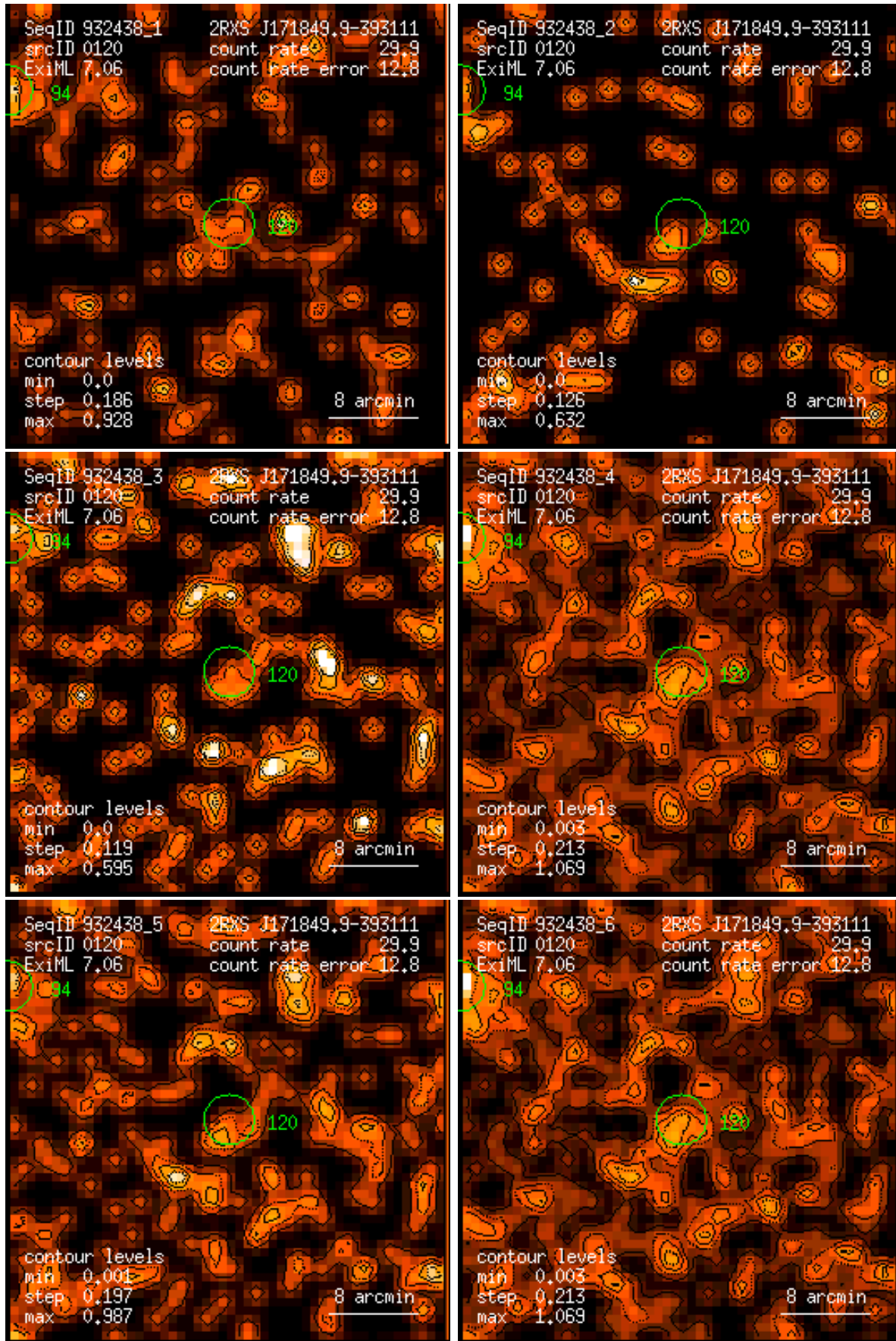
Figure 120: RASS 932438: detection 0120: band rate images, Gaussian filter: (1) PSPC channels 11 – 41, (2) 52 – 90, (3) 91 – 201, (4) 11 – 235, (5) 52 – 201, (6) 11 – 201. Broad band rates in counts/ks. Band rate contour levels in counts/ks/arcmin 2 .
