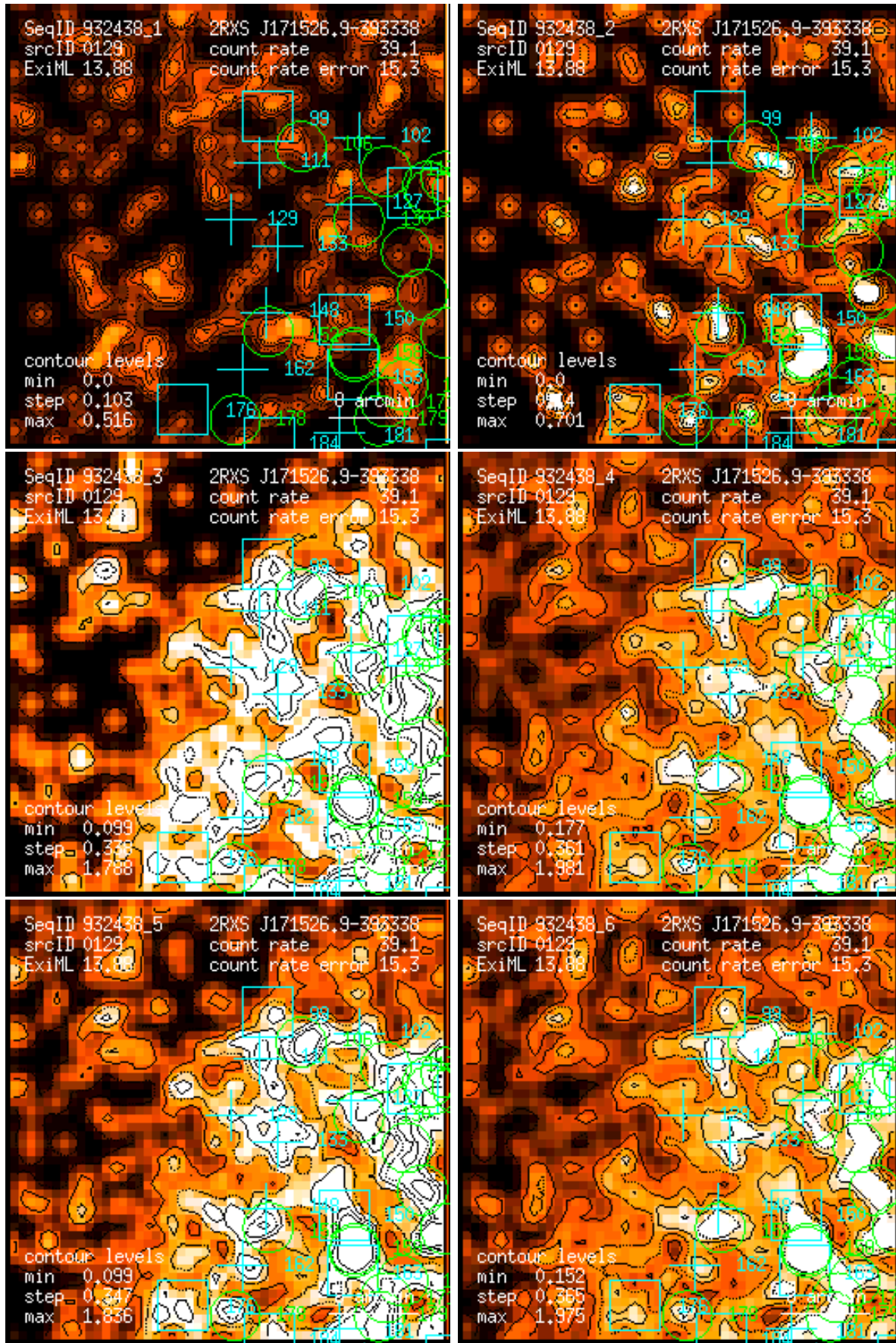
Figure 129: RASS 932438: detection 0129: band rate images, Gaussian filter: (1) PSPC channels 11 – 41, (2) 52 – 90, (3) 91 – 201, (4) 11 – 235, (5) 52 – 201, (6) 11 – 201. Broad band rates in counts/ks. Band rate contour levels in counts/ks/arcmin 2 .
