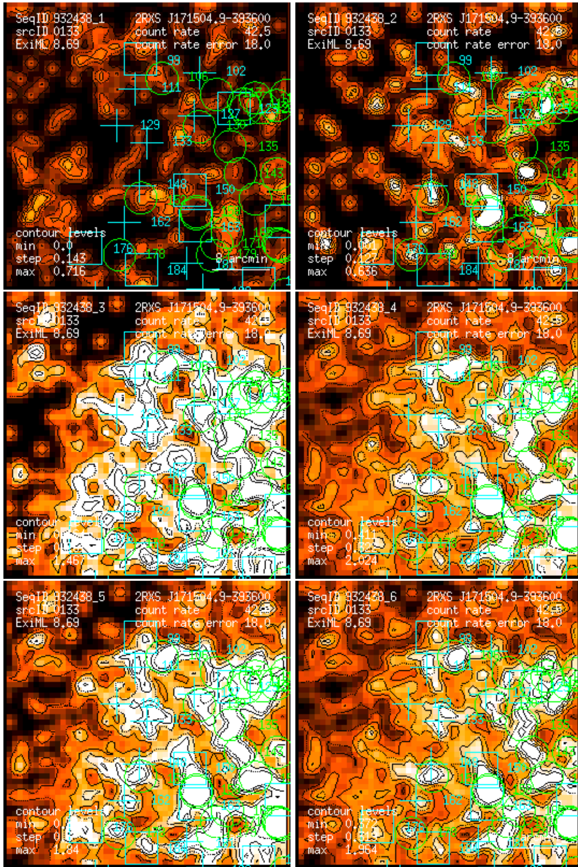
Figure 133: RASS 932438: detection 0133: band rate images, Gaussian filter: (1) PSPC channels 11 – 41, (2) 52 – 90, (3) 91 – 201, (4) 11 – 235, (5) 52 – 201, (6) 11 – 201. Broad band rates in counts/ks. Band rate contour levels in counts/ks/arcmin 2 .
