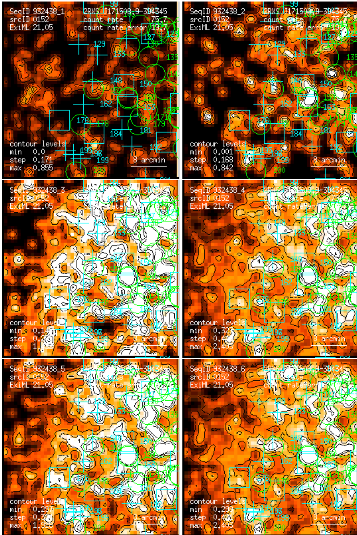
Figure 152: RASS 932438: detection 0152: band rate images, Gaussian filter: (1) PSPC channels 11 – 41, (2) 52 – 90, (3) 91 – 201, (4) 11 – 235, (5) 52 – 201, (6) 11 – 201. Broad band rates in counts/ks. Band rate contour levels in counts/ks/arcmin 2 .
