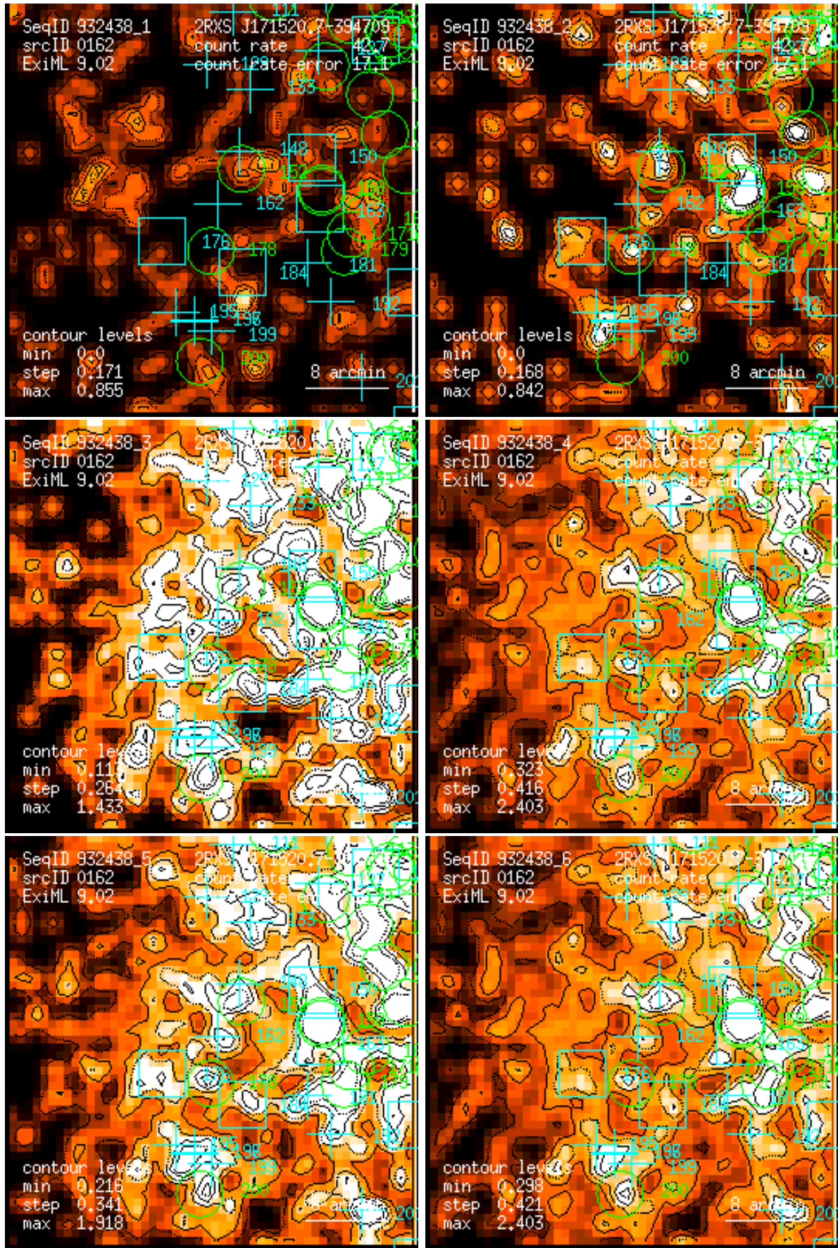
Figure 162: RASS 932438: detection 0162: band rate images, Gaussian filter: (1) PSPC channels 11 – 41, (2) 52 – 90, (3) 91 – 201, (4) 11 – 235, (5) 52 – 201, (6) 11 – 201. Broad band rates in counts/ks. Band rate contour levels in counts/ks/arcmin 2 .
