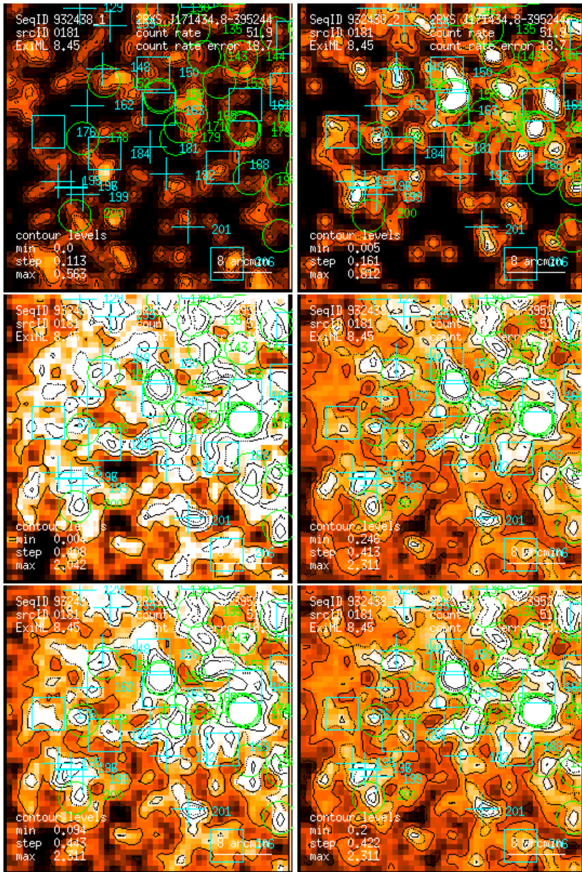
Figure 181: RASS 932438: detection 0181: band rate images, Gaussian filter: (1) PSPC channels 11 – 41, (2) 52 – 90, (3) 91 – 201, (4) 11 – 235, (5) 52 – 201, (6) 11 – 201. Broad band rates in counts/ks. Band rate contour levels in counts/ks/arcmin 2 .
