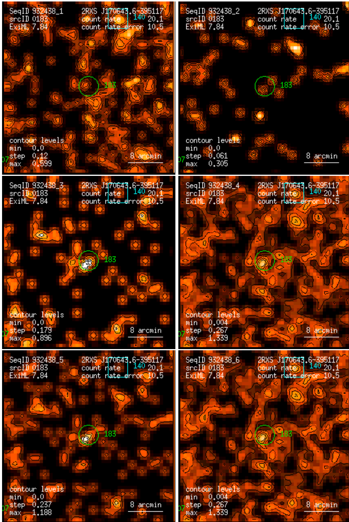
Figure 183: RASS 932438: detection 0183: band rate images, Gaussian filter: (1) PSPC channels 11 – 41, (2) 52 – 90, (3) 91 – 201, (4) 11 – 235, (5) 52 – 201, (6) 11 – 201. Broad band rates in counts/ks. Band rate contour levels in counts/ks/arcmin 2 .
