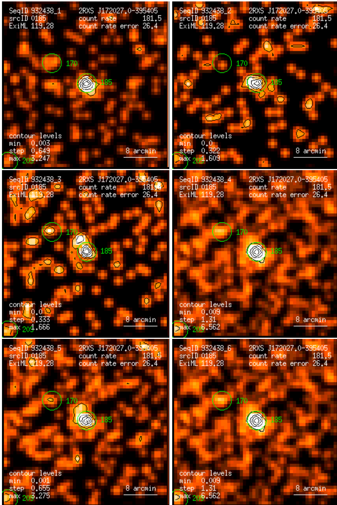
Figure 185: RASS 932438: detection 0185: band rate images, Gaussian filter: (1) PSPC channels 11 – 41, (2) 52 – 90, (3) 91 – 201, (4) 11 – 235, (5) 52 – 201, (6) 11 – 201. Broad band rates in counts/ks. Band rate contour levels in counts/ks/arcmin 2 .
