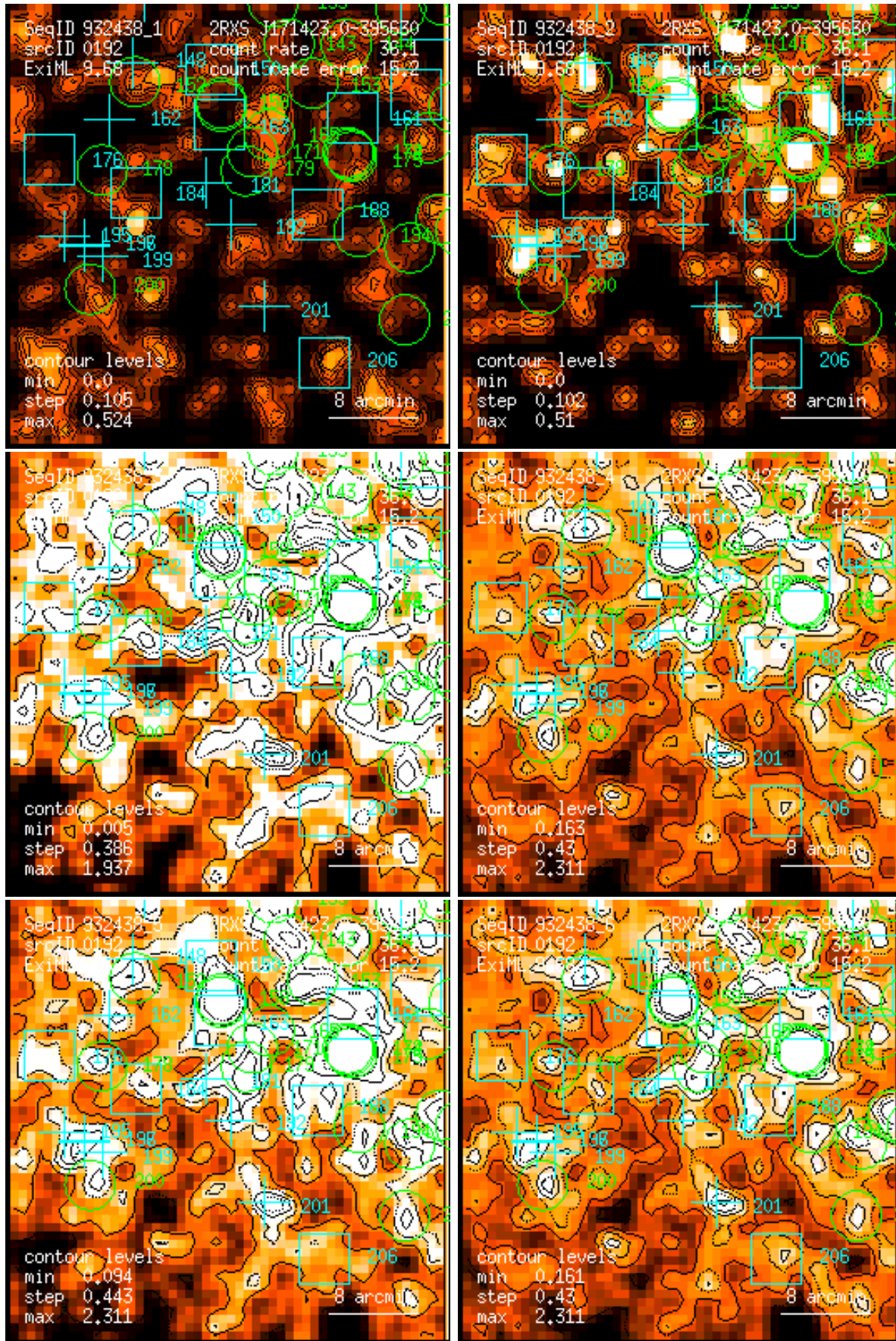
Figure 192: RASS 932438: detection 0192: band rate images, Gaussian filter: (1) PSPC channels 11 – 41, (2) 52 – 90, (3) 91 – 201, (4) 11 – 235, (5) 52 – 201, (6) 11 – 201. Broad band rates in counts/ks. Band rate contour levels in counts/ks/arcmin 2 .
