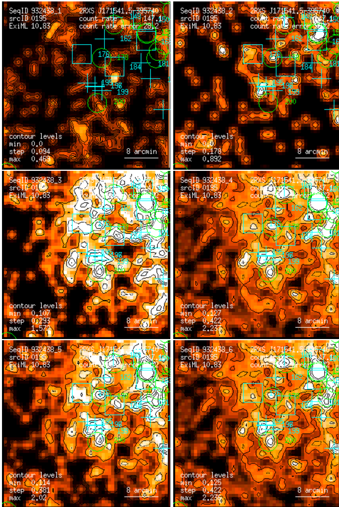
Figure 195: RASS 932438: detection 0195: band rate images, Gaussian filter: (1) PSPC channels 11 – 41, (2) 52 – 90, (3) 91 – 201, (4) 11 – 235, (5) 52 – 201, (6) 11 – 201. Broad band rates in counts/ks. Band rate contour levels in counts/ks/arcmin 2 .
