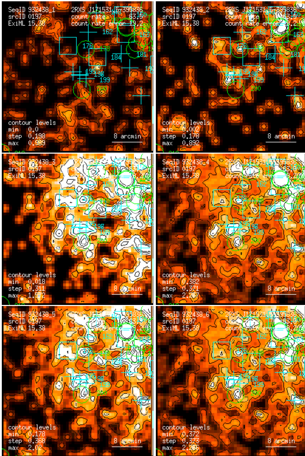
Figure 197: RASS 932438: detection 0197: band rate images, Gaussian filter: (1) PSPC channels 11 – 41, (2) 52 – 90, (3) 91 – 201, (4) 11 – 235, (5) 52 – 201, (6) 11 – 201. Broad band rates in counts/ks. Band rate contour levels in counts/ks/arcmin 2 .
