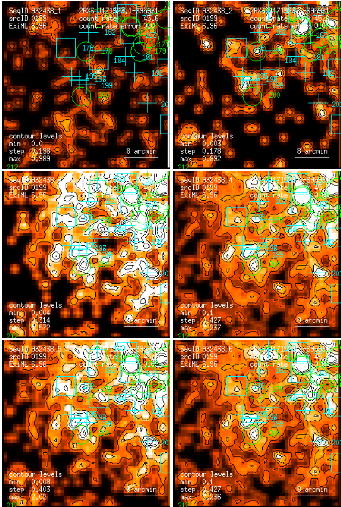
Figure 199: RASS 932438: detection 0199: band rate images, Gaussian filter: (1) PSPC channels 11 – 41, (2) 52 – 90, (3) 91 – 201, (4) 11 – 235, (5) 52 – 201, (6) 11 – 201. Broad band rates in counts/ks. Band rate contour levels in counts/ks/arcmin 2 .
