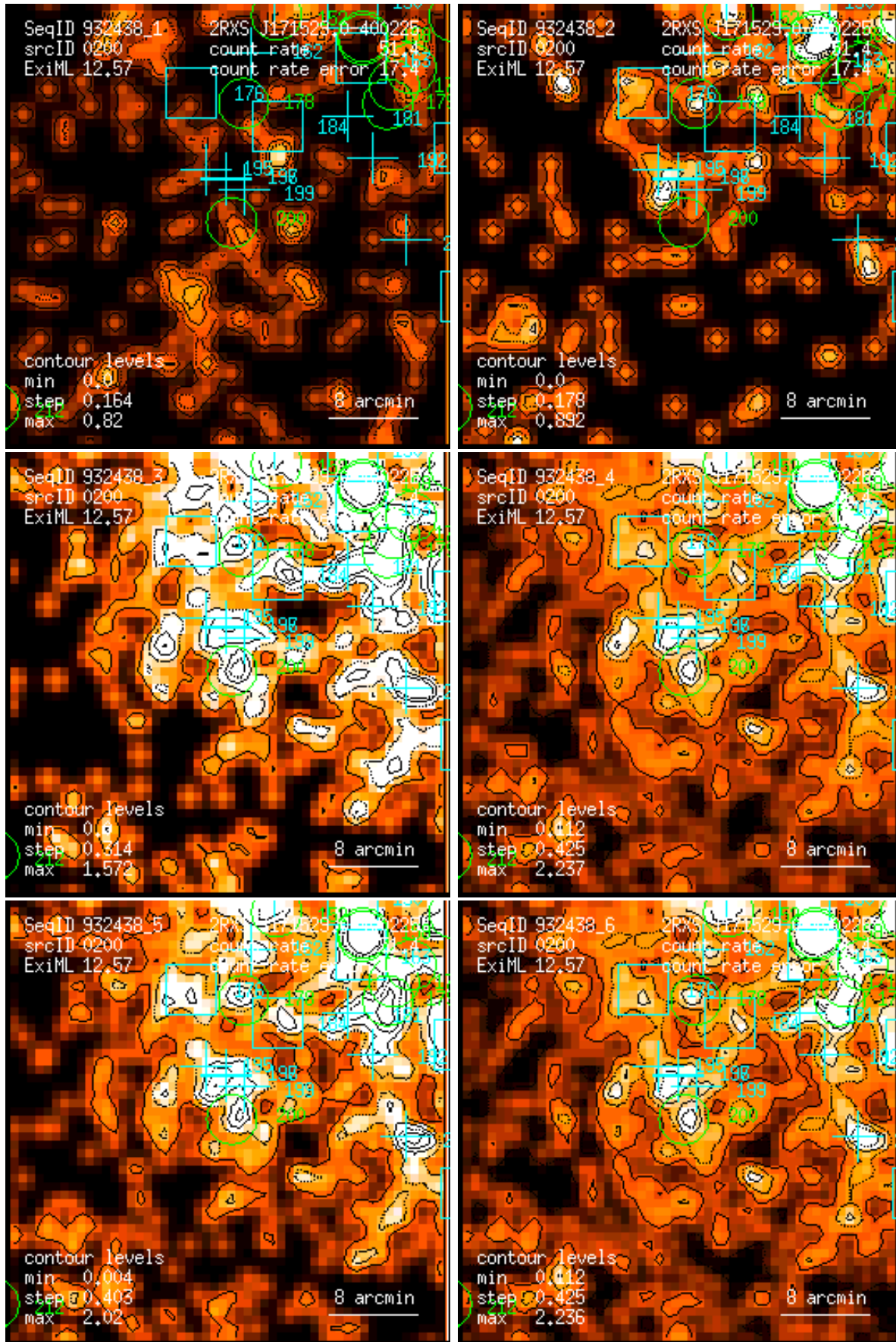
Figure 200: RASS 932438: detection 0200: band rate images, Gaussian filter: (1) PSPC channels 11 – 41, (2) 52 – 90, (3) 91 – 201, (4) 11 – 235, (5) 52 – 201, (6) 11 – 201. Broad band rates in counts/ks. Band rate contour levels in counts/ks/arcmin 2 .
