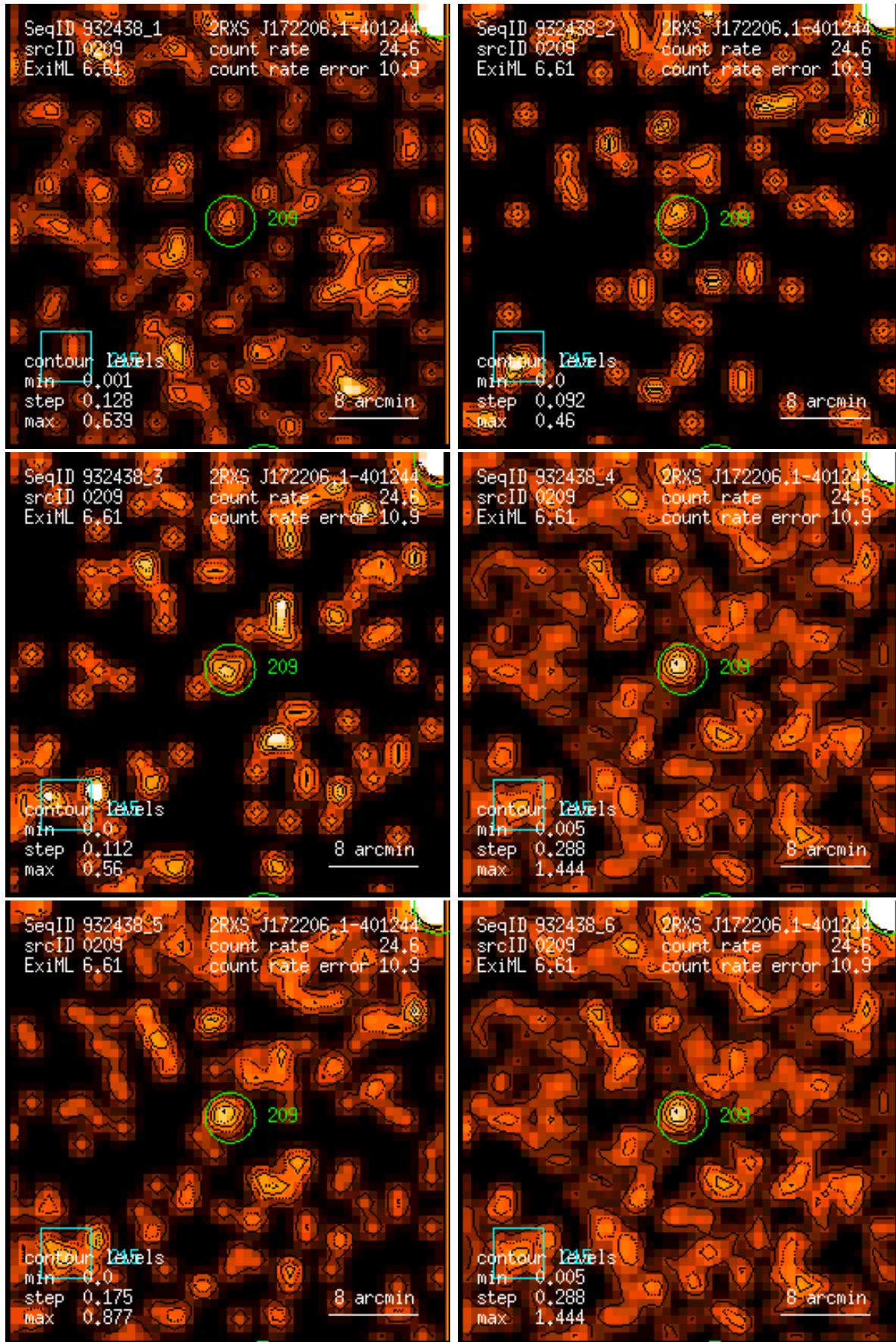
Figure 209: RASS 932438: detection 0209: band rate images, Gaussian filter: (1) PSPC channels 11 – 41, (2) 52 – 90, (3) 91 – 201, (4) 11 – 235, (5) 52 – 201, (6) 11 – 201. Broad band rates in counts/ks. Band rate contour levels in counts/ks/arcmin 2 .
