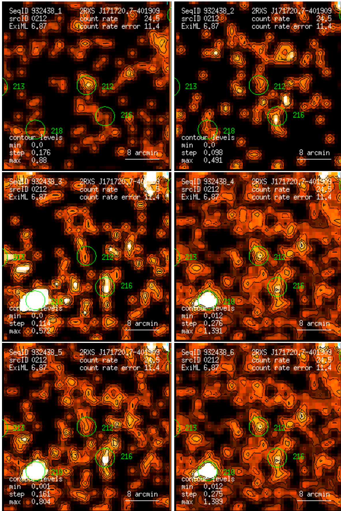
Figure 212: RASS 932438: detection 0212: band rate images, Gaussian filter: (1) PSPC channels 11 – 41, (2) 52 – 90, (3) 91 – 201, (4) 11 – 235, (5) 52 – 201, (6) 11 – 201. Broad band rates in counts/ks. Band rate contour levels in counts/ks/arcmin 2 .
