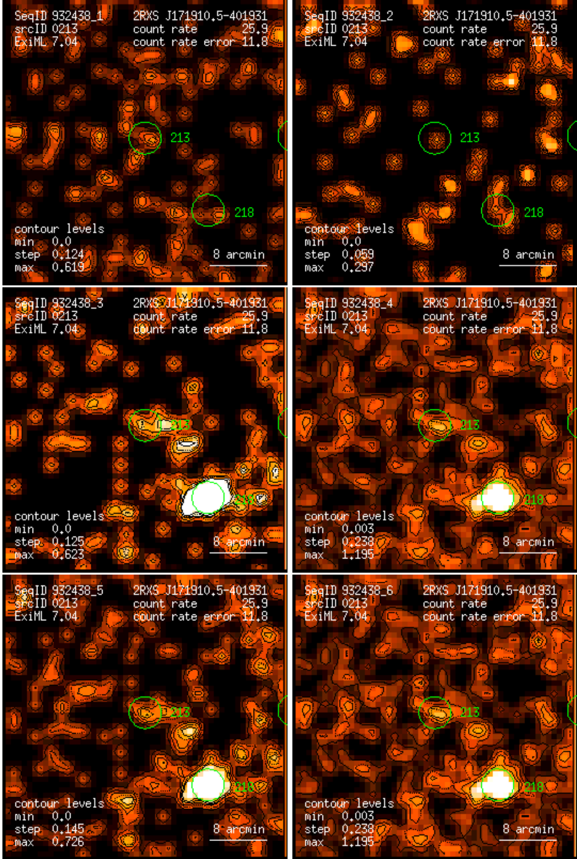
Figure 213: RASS 932438: detection 0213: band rate images, Gaussian filter: (1) PSPC channels 11 – 41, (2) 52 – 90, (3) 91 – 201, (4) 11 – 235, (5) 52 – 201, (6) 11 – 201. Broad band rates in counts/ks. Band rate contour levels in counts/ks/arcmin 2 .
