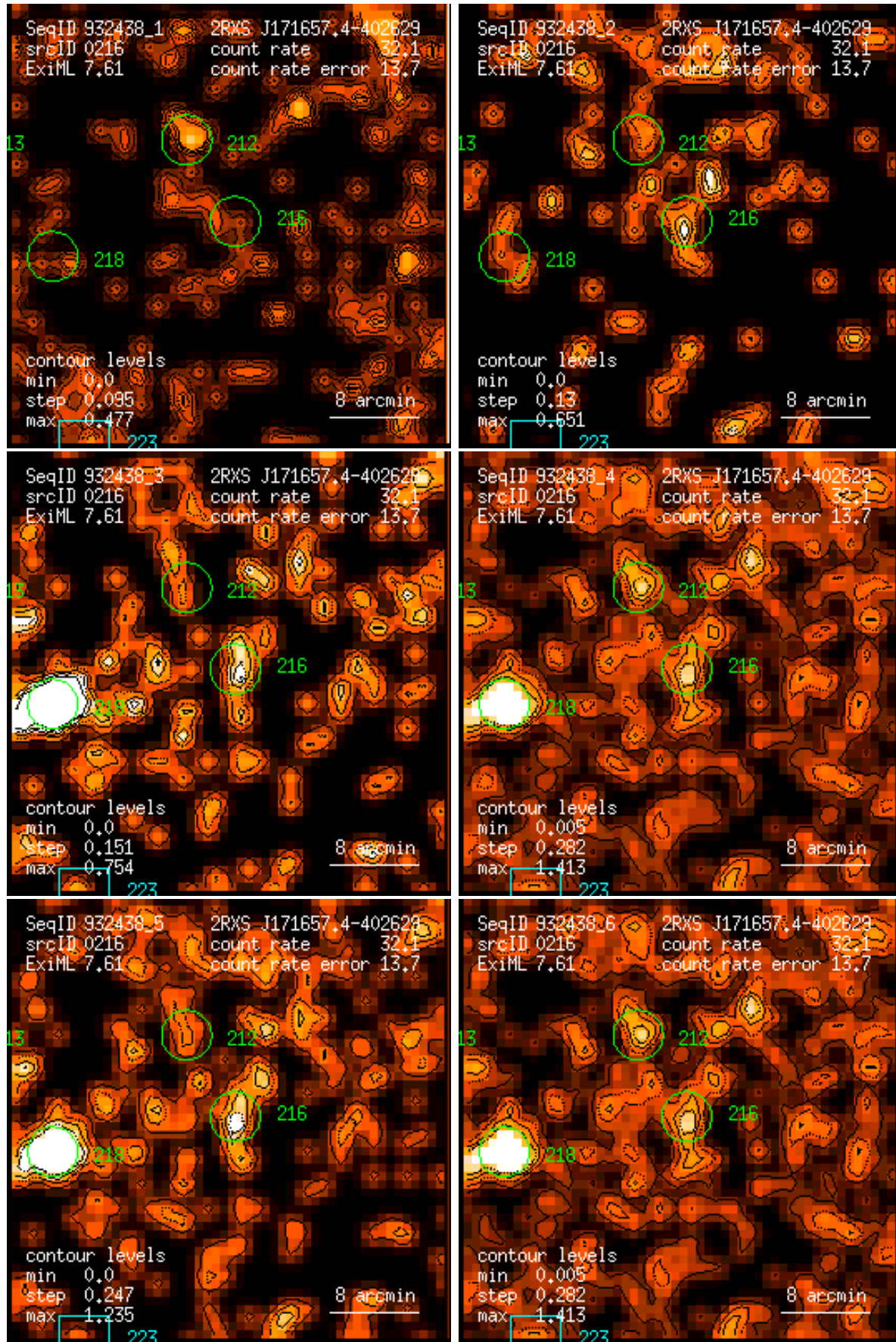
Figure 216: RASS 932438: detection 0216: band rate images, Gaussian filter: (1) PSPC channels 11 – 41, (2) 52 – 90, (3) 91 – 201, (4) 11 – 235, (5) 52 – 201, (6) 11 – 201. Broad band rates in counts/ks. Band rate contour levels in counts/ks/arcmin 2 .
