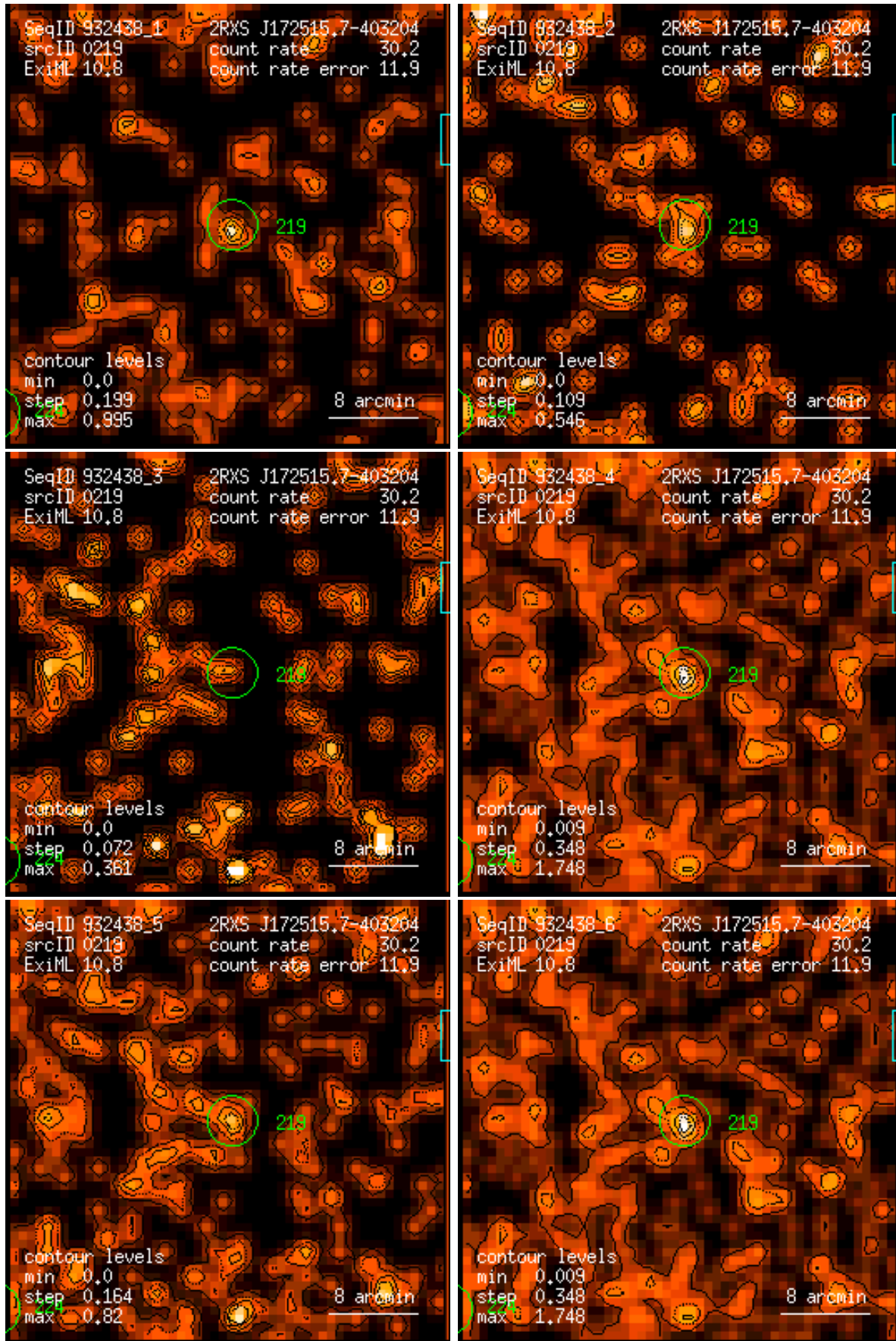
Figure 219: RASS 932438: detection 0219: band rate images, Gaussian filter: (1) PSPC channels 11 – 41, (2) 52 – 90, (3) 91 – 201, (4) 11 – 235, (5) 52 – 201, (6) 11 – 201. Broad band rates in counts/ks. Band rate contour levels in counts/ks/arcmin 2 .
