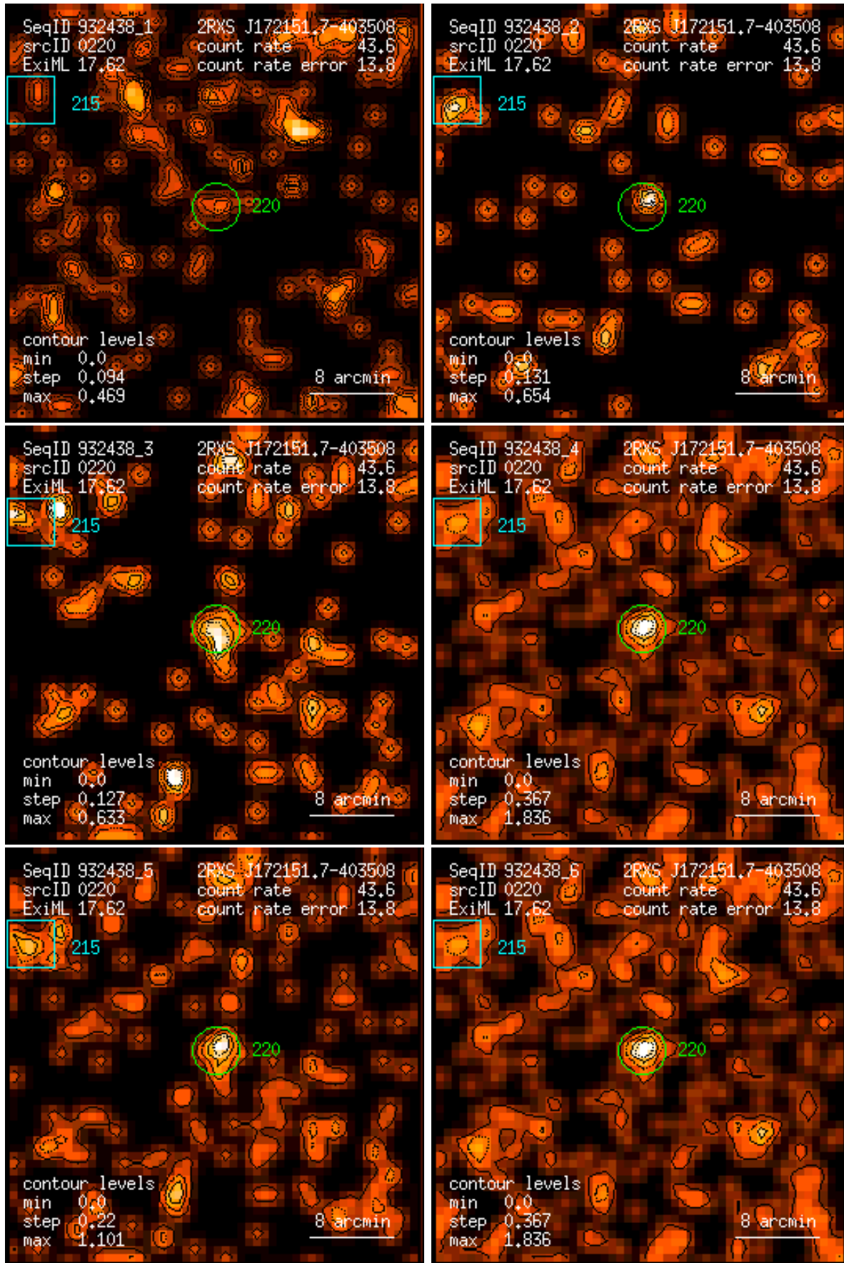
Figure 220: RASS 932438: detection 0220: band rate images, Gaussian filter: (1) PSPC channels 11 – 41, (2) 52 – 90, (3) 91 – 201, (4) 11 – 235, (5) 52 – 201, (6) 11 – 201. Broad band rates in counts/ks. Band rate contour levels in counts/ks/arcmin 2 .
