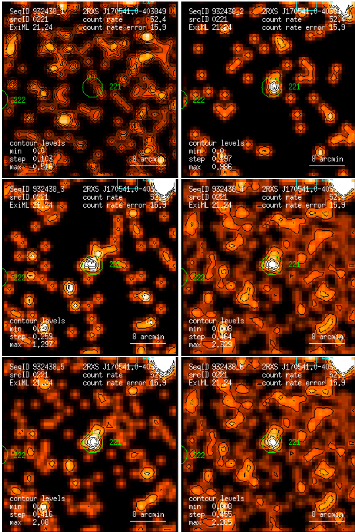
Figure 221: RASS 932438: detection 0221: band rate images, Gaussian filter: (1) PSPC channels 11 – 41, (2) 52 – 90, (3) 91 – 201, (4) 11 – 235, (5) 52 – 201, (6) 11 – 201. Broad band rates in counts/ks. Band rate contour levels in counts/ks/arcmin 2 .
