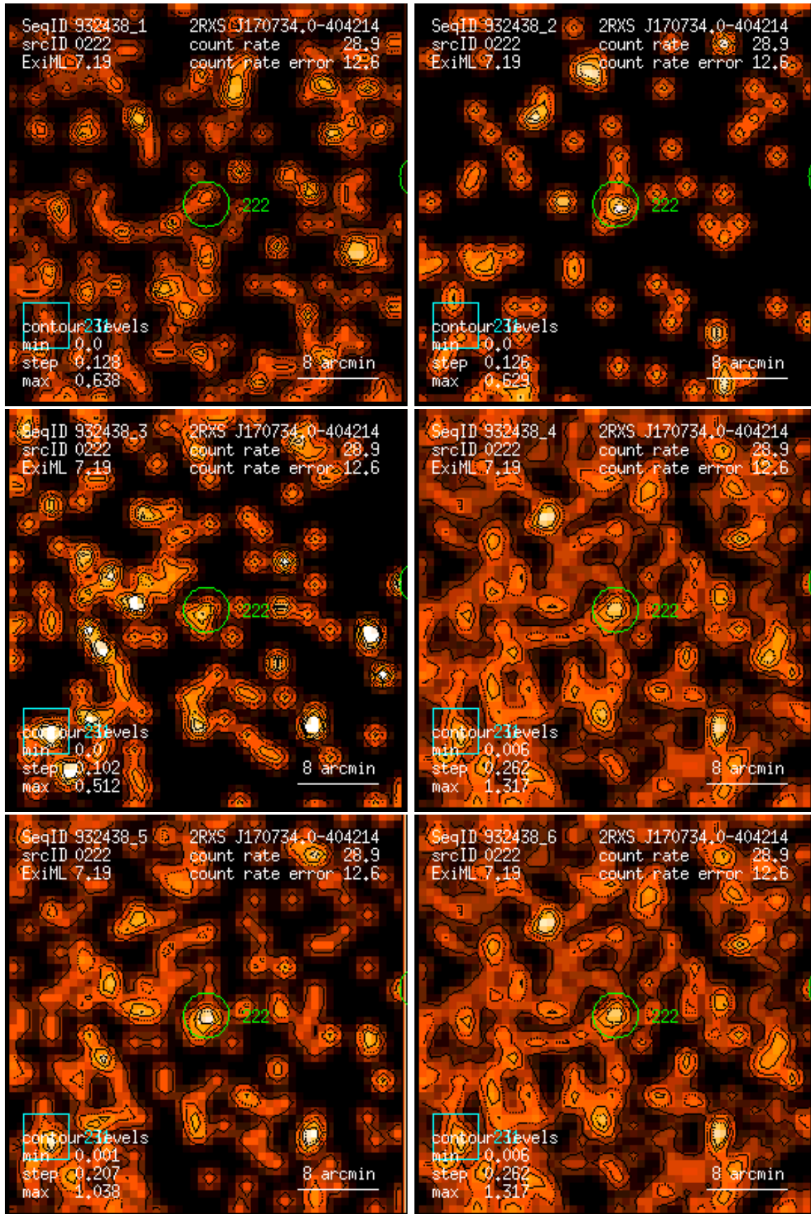
Figure 222: RASS 932438: detection 0222: band rate images, Gaussian filter: (1) PSPC channels 11 – 41, (2) 52 – 90, (3) 91 – 201, (4) 11 – 235, (5) 52 – 201, (6) 11 – 201. Broad band rates in counts/ks. Band rate contour levels in counts/ks/arcmin 2 .
