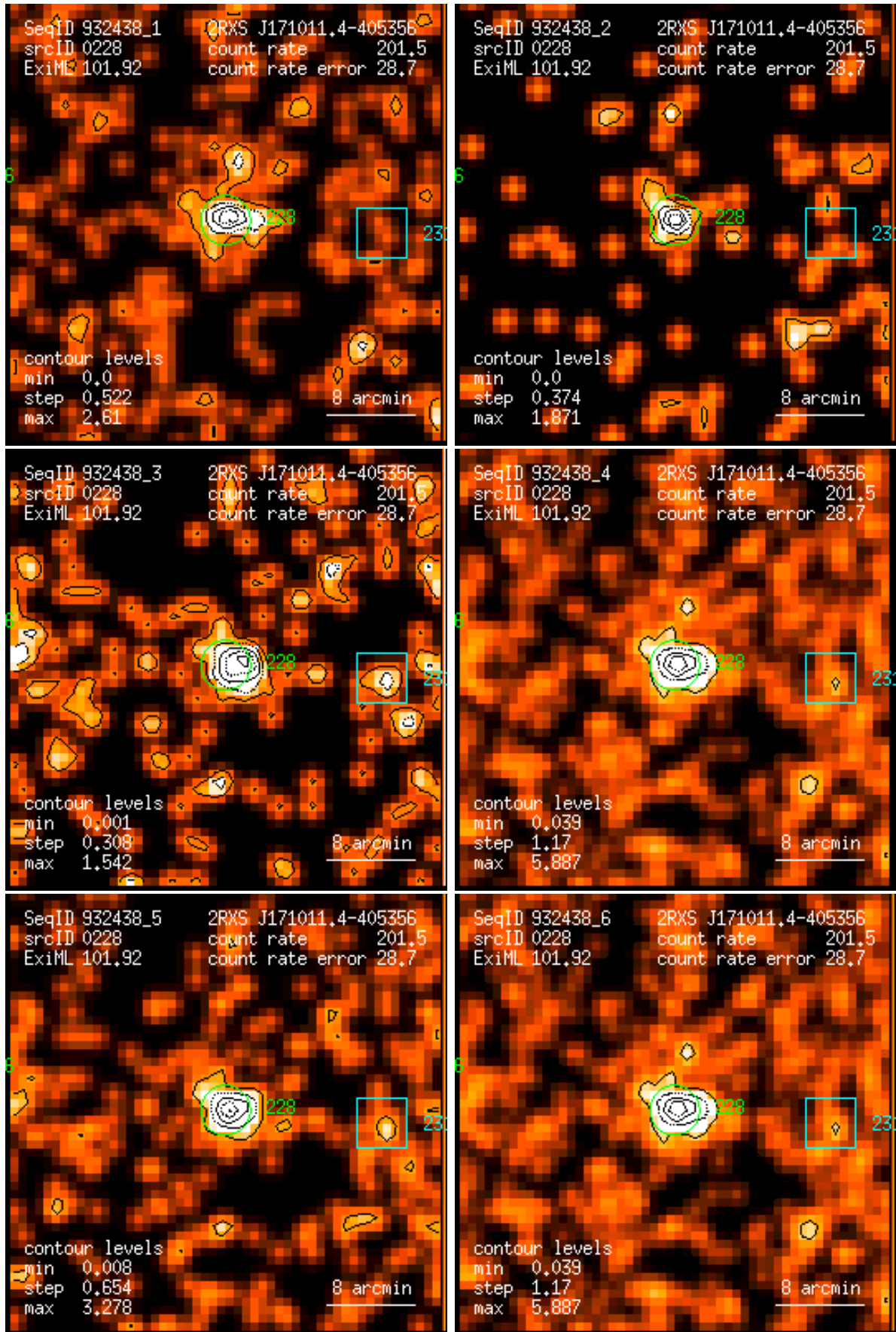
Figure 228: RASS 932438: detection 0228: band rate images, Gaussian filter: (1) PSPC channels 11 – 41, (2) 52 – 90, (3) 91 – 201, (4) 11 – 235, (5) 52 – 201, (6) 11 – 201. Broad band rates in counts/ks. Band rate contour levels in counts/ks/arcmin 2 .
