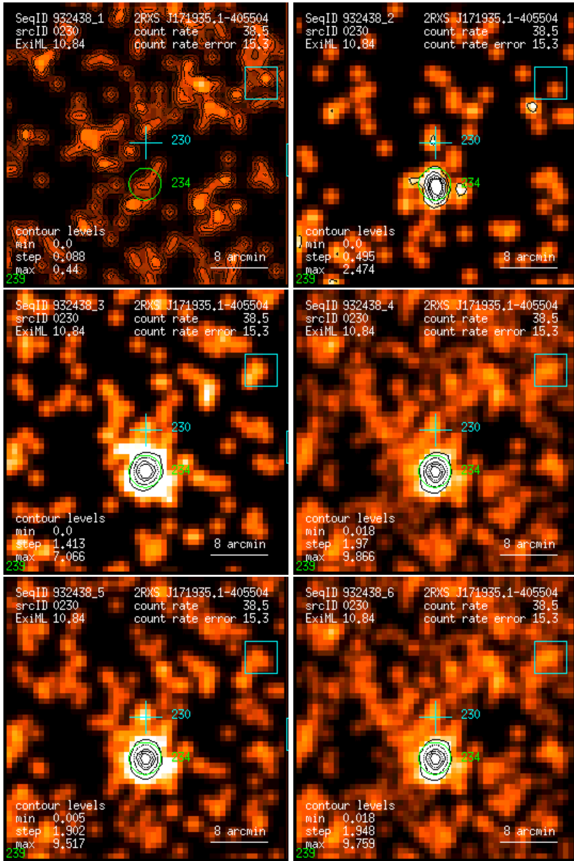
Figure 230: RASS 932438: detection 0230: band rate images, Gaussian filter: (1) PSPC channels 11 – 41, (2) 52 – 90, (3) 91 – 201, (4) 11 – 235, (5) 52 – 201, (6) 11 – 201. Broad band rates in counts/ks. Band rate contour levels in counts/ks/arcmin 2 .
