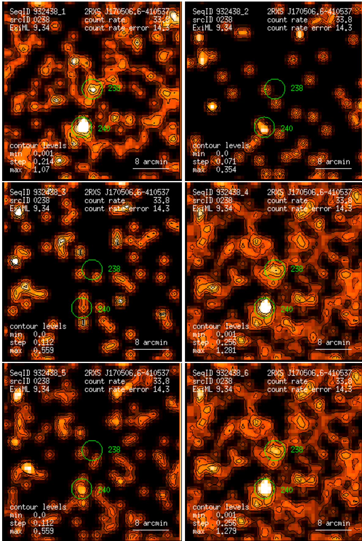
Figure 238: RASS 932438: detection 0238: band rate images, Gaussian filter: (1) PSPC channels 11 – 41, (2) 52 – 90, (3) 91 – 201, (4) 11 – 235, (5) 52 – 201, (6) 11 – 201. Broad band rates in counts/ks. Band rate contour levels in counts/ks/arcmin 2 .
