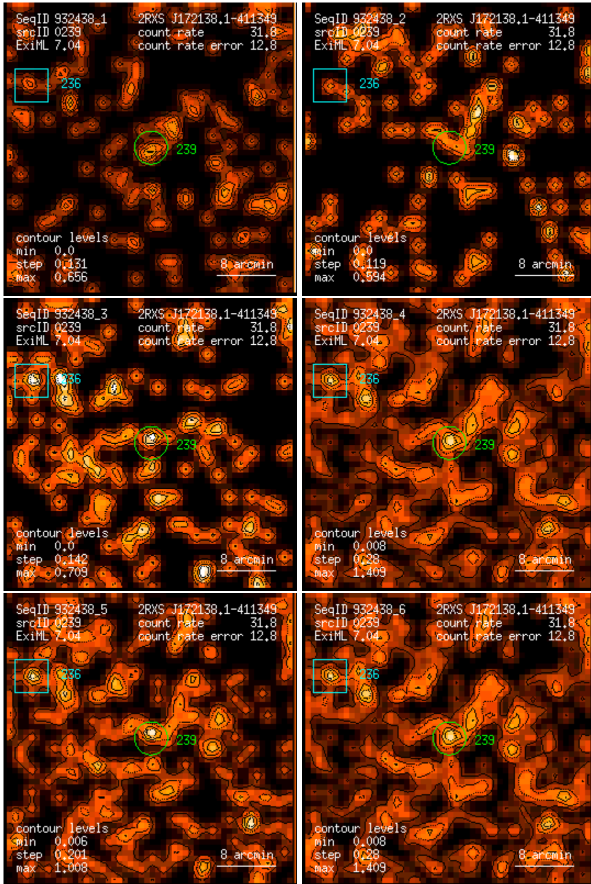
Figure 239: RASS 932438: detection 0239: band rate images, Gaussian filter: (1) PSPC channels 11 – 41, (2) 52 – 90, (3) 91 – 201, (4) 11 – 235, (5) 52 – 201, (6) 11 – 201. Broad band rates in counts/ks. Band rate contour levels in counts/ks/arcmin 2 .
