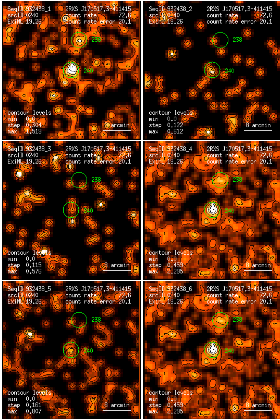
Figure 240: RASS 932438: detection 0240: band rate images, Gaussian filter: (1) PSPC channels 11 – 41, (2) 52 – 90, (3) 91 – 201, (4) 11 – 235, (5) 52 – 201, (6) 11 – 201. Broad band rates in counts/ks. Band rate contour levels in counts/ks/arcmin 2 .
