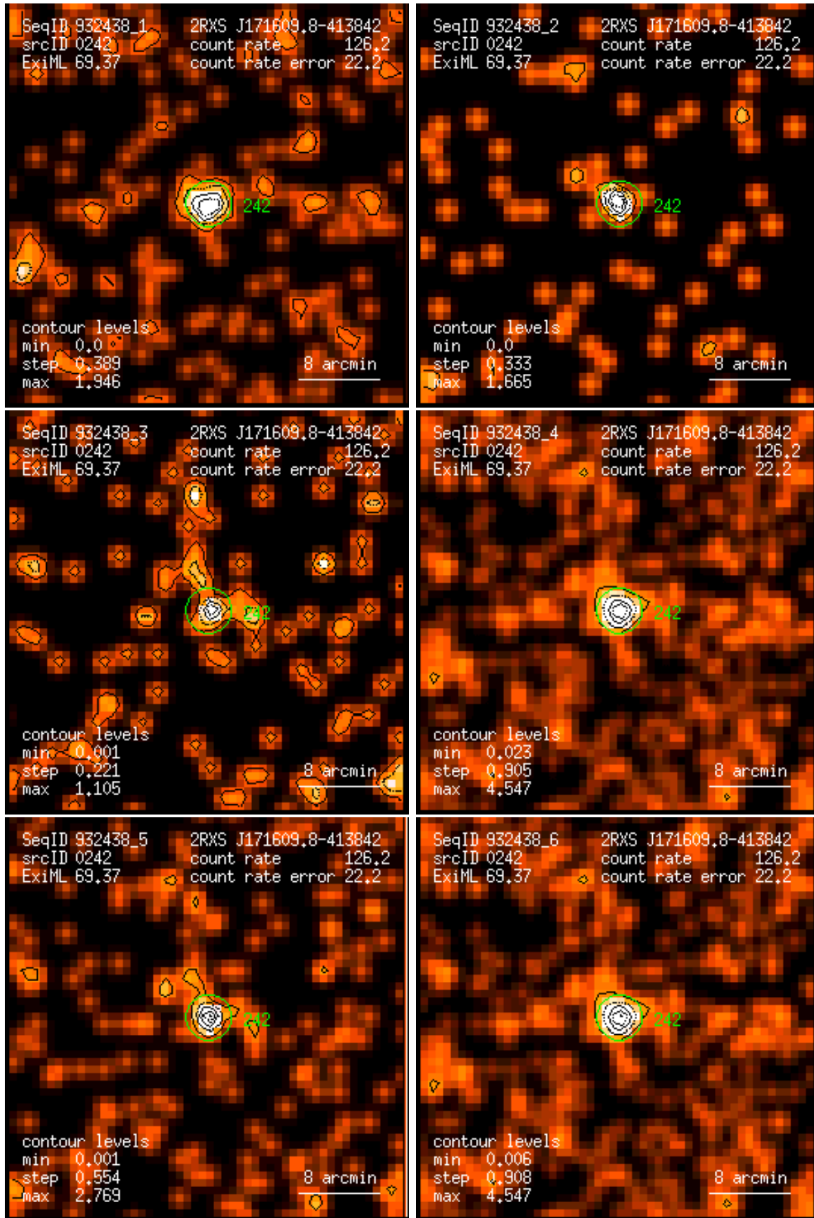
Figure 242: RASS 932438: detection 0242: band rate images, Gaussian filter: (1) PSPC channels 11 – 41, (2) 52 – 90, (3) 91 – 201, (4) 11 – 235, (5) 52 – 201, (6) 11 – 201. Broad band rates in counts/ks. Band rate contour levels in counts/ks/arcmin 2 .
