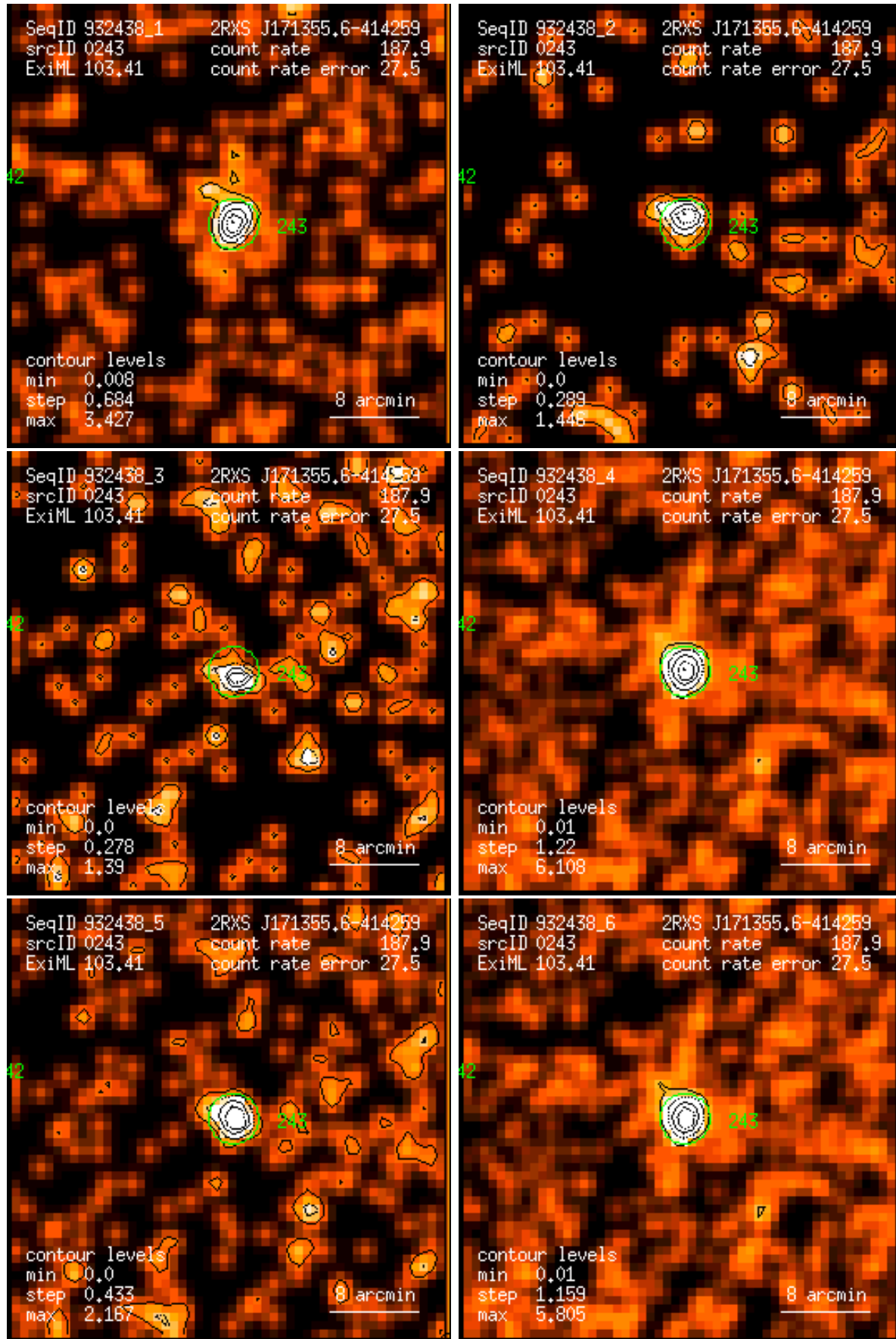
Figure 243: RASS 932438: detection 0243: band rate images, Gaussian filter: (1) PSPC channels 11 – 41, (2) 52 – 90, (3) 91 – 201, (4) 11 – 235, (5) 52 – 201, (6) 11 – 201. Broad band rates in counts/ks. Band rate contour levels in counts/ks/arcmin 2 .
