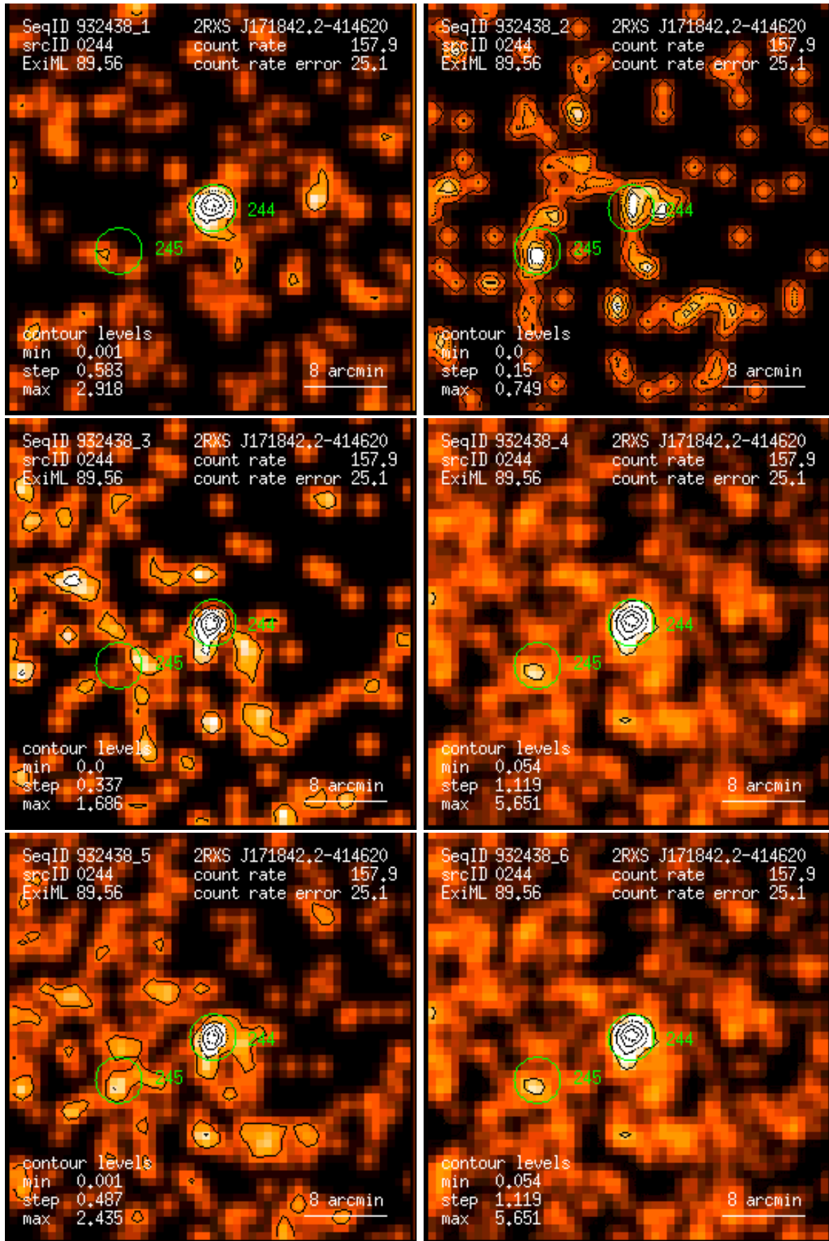
Figure 244: RASS 932438: detection 0244: band rate images, Gaussian filter: (1) PSPC channels 11 – 41, (2) 52 – 90, (3) 91 – 201, (4) 11 – 235, (5) 52 – 201, (6) 11 – 201. Broad band rates in counts/ks. Band rate contour levels in counts/ks/arcmin 2 .
