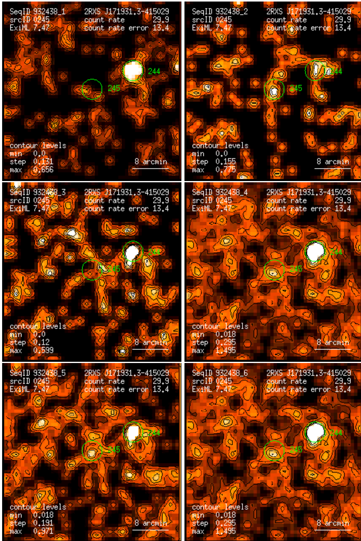
Figure 245: RASS 932438: detection 0245: band rate images, Gaussian filter: (1) PSPC channels 11 – 41, (2) 52 – 90, (3) 91 – 201, (4) 11 – 235, (5) 52 – 201, (6) 11 – 201. Broad band rates in counts/ks. Band rate contour levels in counts/ks/arcmin 2 .
