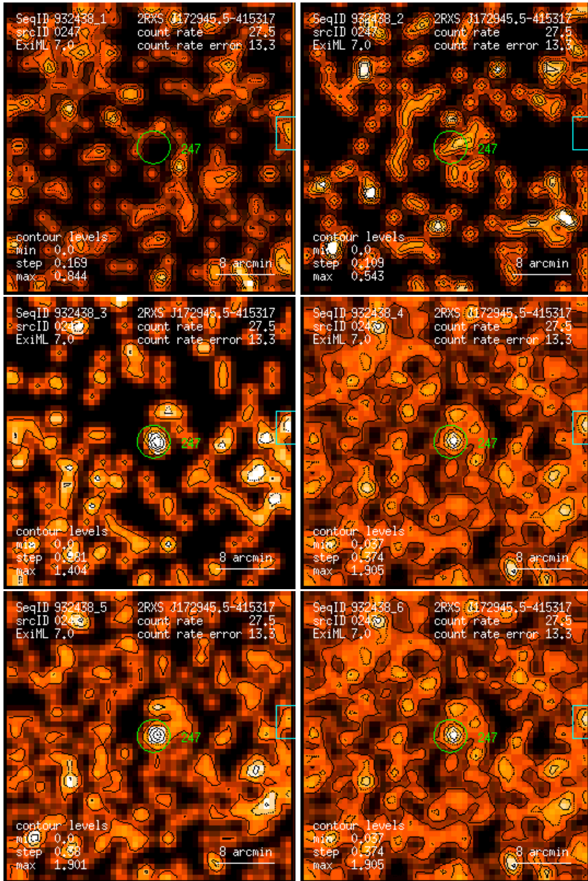
Figure 247: RASS 932438: detection 0247: band rate images, Gaussian filter: (1) PSPC channels 11 – 41, (2) 52 – 90, (3) 91 – 201, (4) 11 – 235, (5) 52 – 201, (6) 11 – 201. Broad band rates in counts/ks. Band rate contour levels in counts/ks/arcmin 2 .
