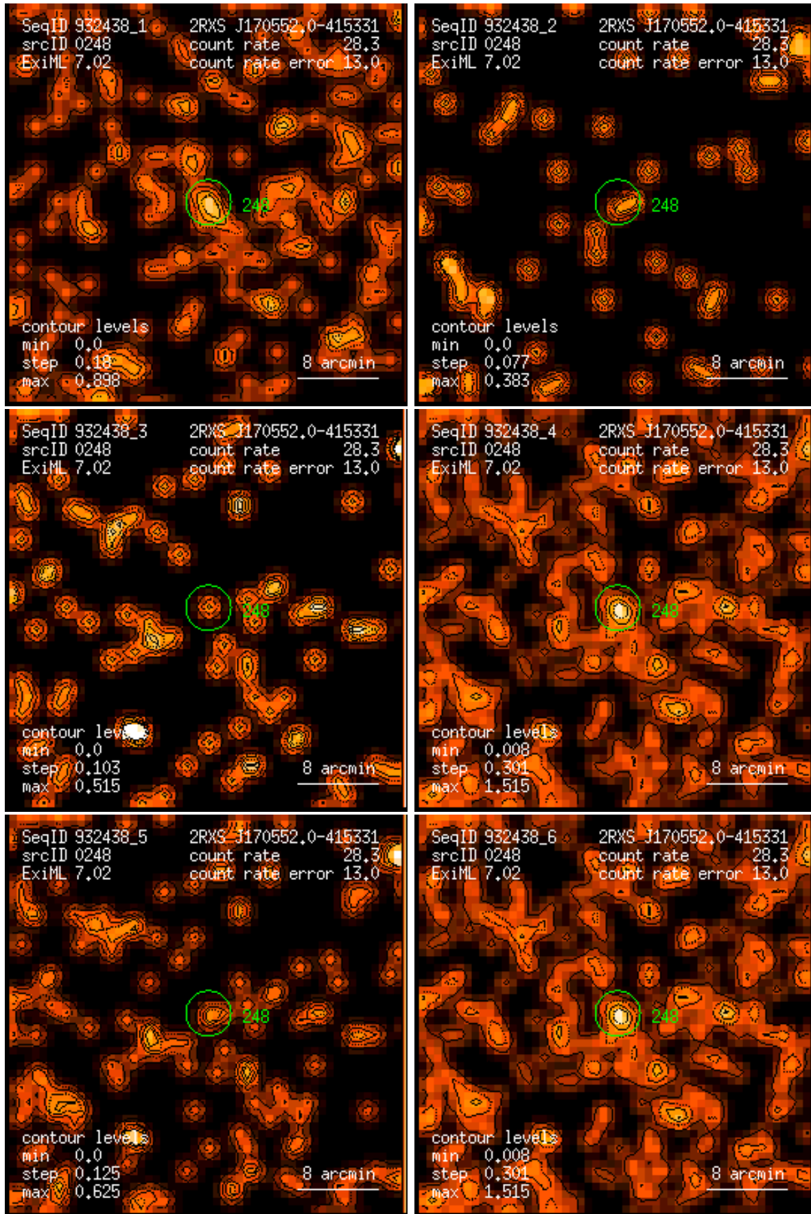
Figure 248: RASS 932438: detection 0248: band rate images, Gaussian filter: (1) PSPC channels 11 – 41, (2) 52 – 90, (3) 91 – 201, (4) 11 – 235, (5) 52 – 201, (6) 11 – 201. Broad band rates in counts/ks. Band rate contour levels in counts/ks/arcmin 2 .
