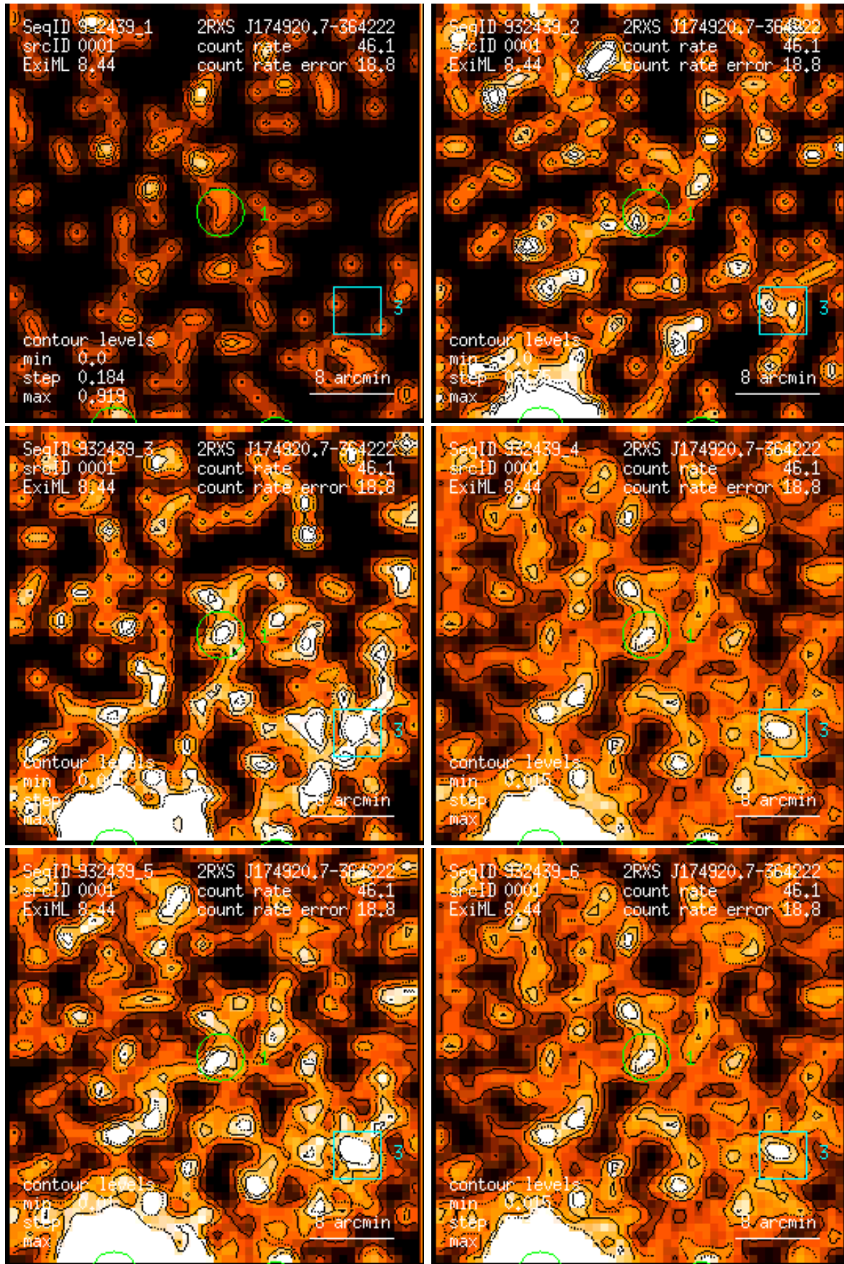
Figure 1: RASS 932439: detection 0001: band rate images, Gaussian filter: (1) PSPC channels 11 – 41, (2) 52 – 90, (3) 91 – 201, (4) 11 – 235, (5) 52 – 201, (6) 11 – 201. Broad band rates in counts/ks. Band rate contour levels in counts/ks/arcmin 2 .
