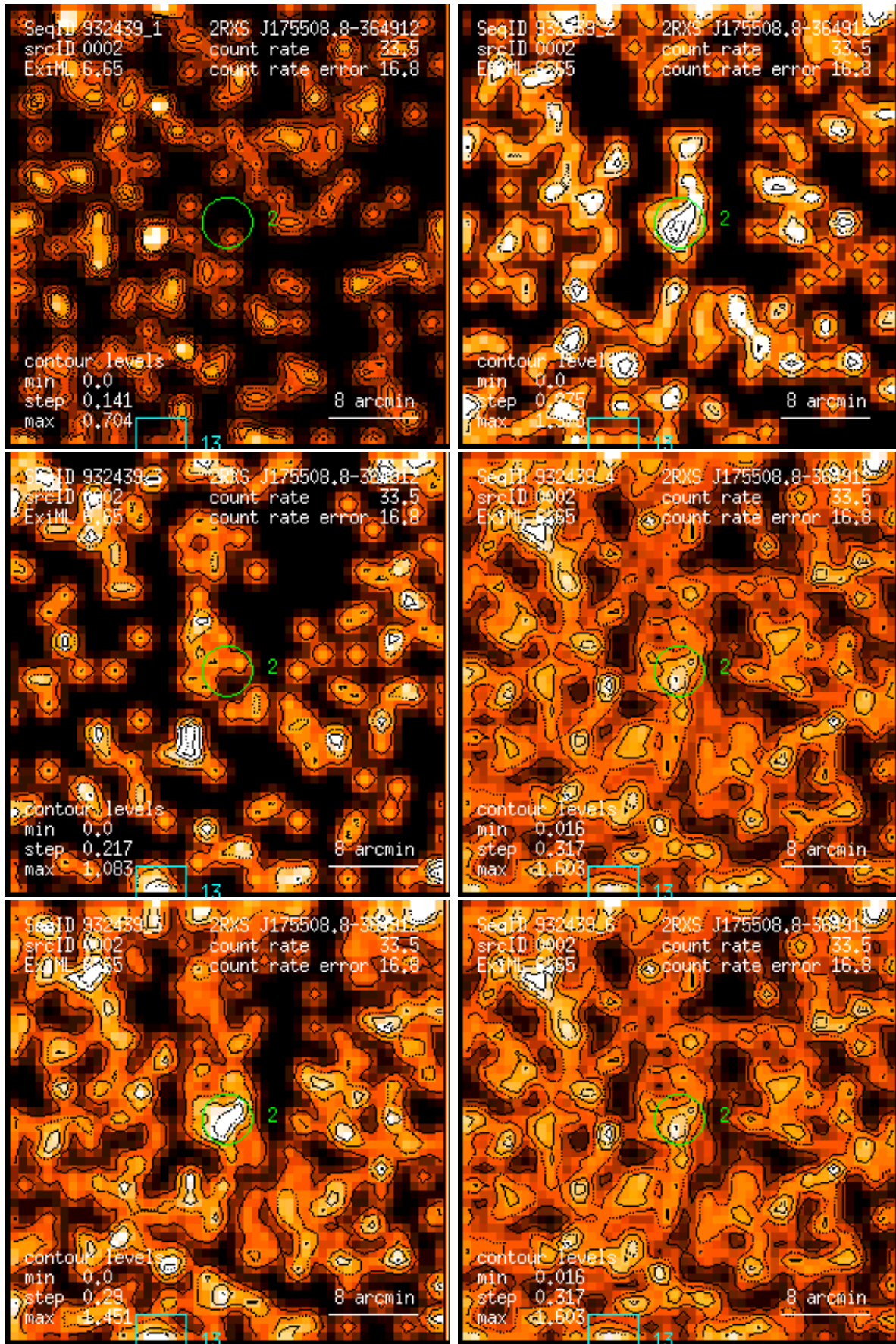
Figure 2: RASS 932439: detection 0002: band rate images, Gaussian filter: (1) PSPC channels 11 – 41, (2) 52 – 90, (3) 91 – 201, (4) 11 – 235, (5) 52 – 201, (6) 11 – 201. Broad band rates in counts/ks. Band rate contour levels in counts/ks/arcmin 2 .
