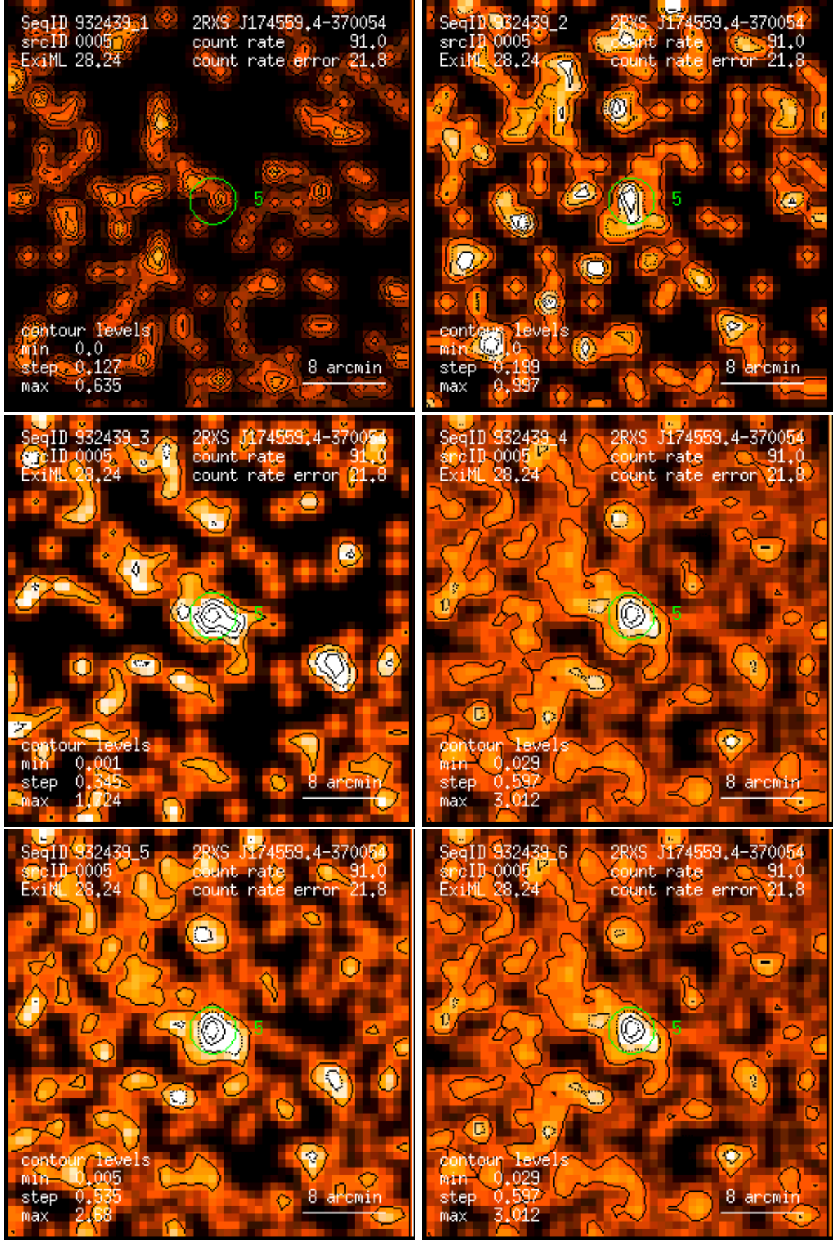
Figure 5: RASS 932439: detection 0005: band rate images, Gaussian filter: (1) PSPC channels 11 – 41, (2) 52 – 90, (3) 91 – 201, (4) 11 – 235, (5) 52 – 201, (6) 11 – 201. Broad band rates in counts/ks. Band rate contour levels in counts/ks/arcmin 2 .
