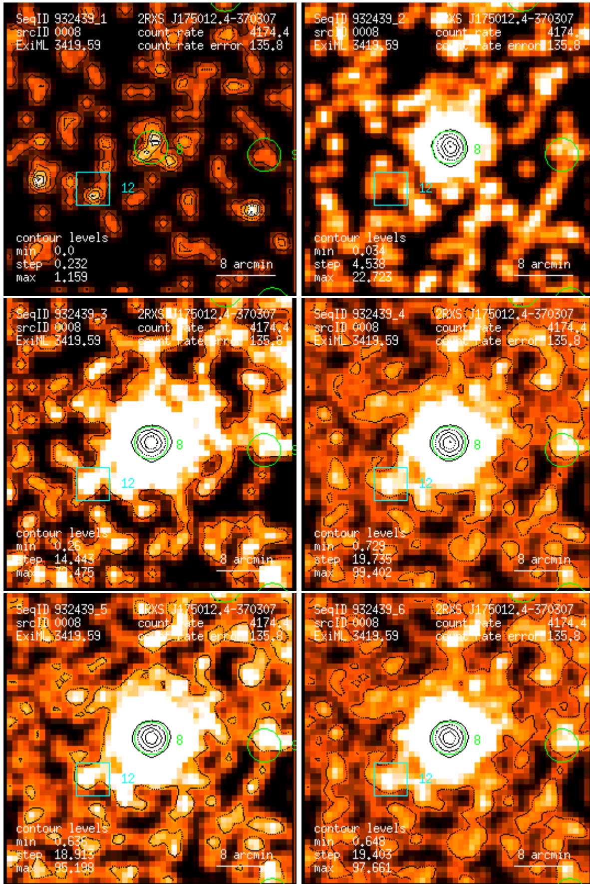
Figure 8: RASS 932439: detection 0008: band rate images, Gaussian filter: (1) PSPC channels 11 – 41, (2) 52 – 90, (3) 91 – 201, (4) 11 – 235, (5) 52 – 201, (6) 11 – 201. Broad band rates in counts/ks. Band rate contour levels in counts/ks/arcmin 2 .
