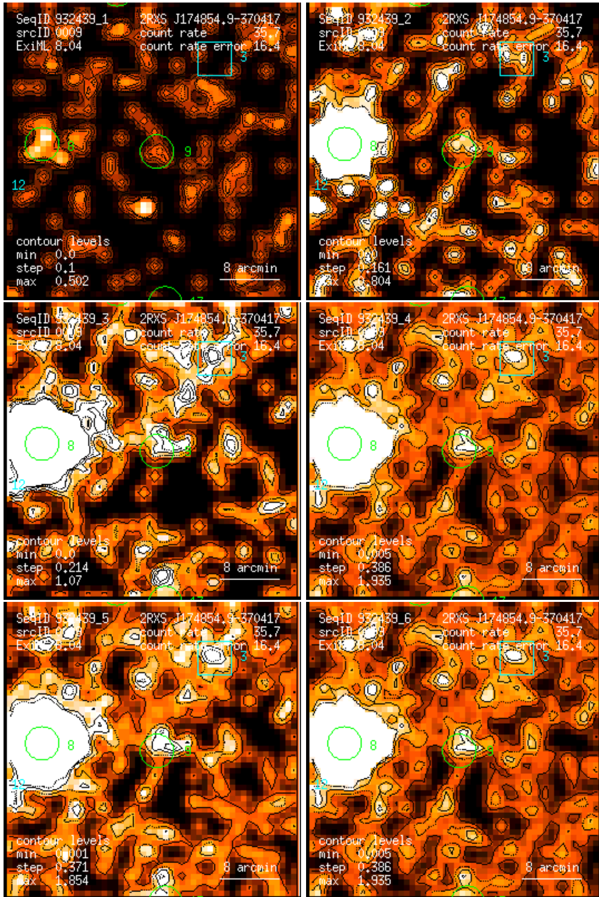
Figure 9: RASS 932439: detection 0009: band rate images, Gaussian filter: (1) PSPC channels 11 – 41, (2) 52 – 90, (3) 91 – 201, (4) 11 – 235, (5) 52 – 201, (6) 11 – 201. Broad band rates in counts/ks. Band rate contour levels in counts/ks/arcmin 2 .
