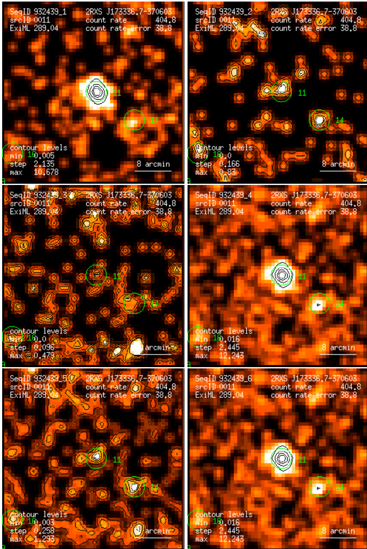
Figure 11: RASS 932439: detection 0011: band rate images, Gaussian filter: (1) PSPC channels 11 – 41, (2) 52 – 90, (3) 91 – 201, (4) 11 – 235, (5) 52 – 201, (6) 11 – 201. Broad band rates in counts/ks. Band rate contour levels in counts/ks/arcmin 2 .
