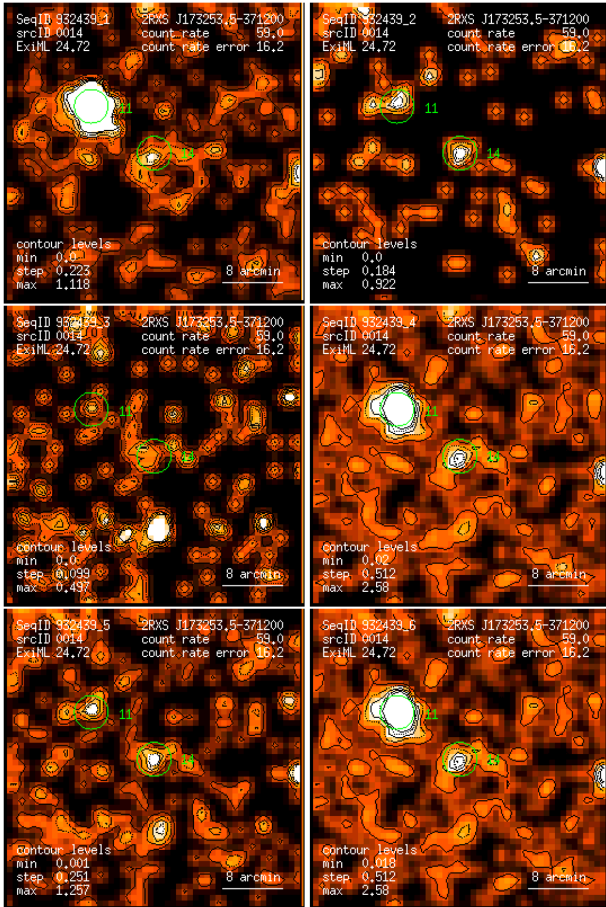
Figure 14: RASS 932439: detection 0014: band rate images, Gaussian filter: (1) PSPC channels 11 – 41, (2) 52 – 90, (3) 91 – 201, (4) 11 – 235, (5) 52 – 201, (6) 11 – 201. Broad band rates in counts/ks. Band rate contour levels in counts/ks/arcmin 2 .
