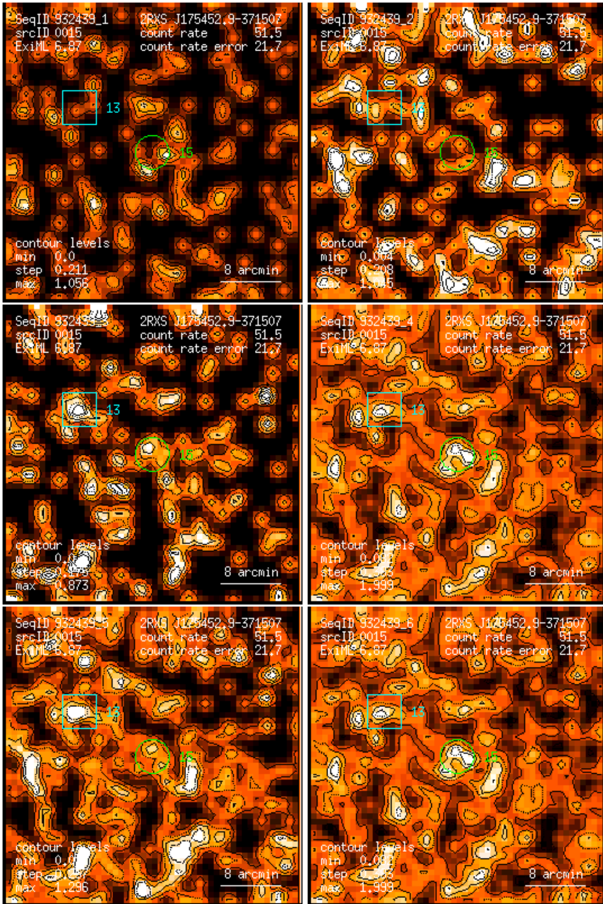
Figure 15: RASS 932439: detection 0015: band rate images, Gaussian filter: (1) PSPC channels 11 – 41, (2) 52 – 90, (3) 91 – 201, (4) 11 – 235, (5) 52 – 201, (6) 11 – 201. Broad band rates in counts/ks. Band rate contour levels in counts/ks/arcmin 2 .
