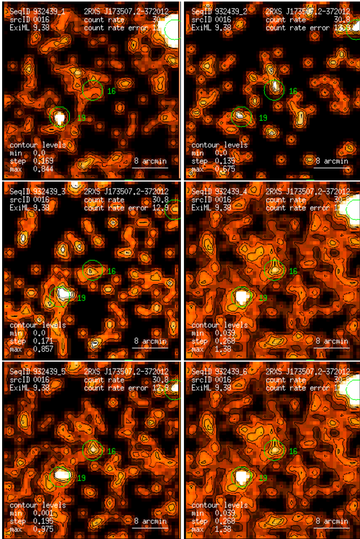
Figure 16: RASS 932439: detection 0016: band rate images, Gaussian filter: (1) PSPC channels 11 – 41, (2) 52 – 90, (3) 91 – 201, (4) 11 – 235, (5) 52 – 201, (6) 11 – 201. Broad band rates in counts/ks. Band rate contour levels in counts/ks/arcmin 2 .
