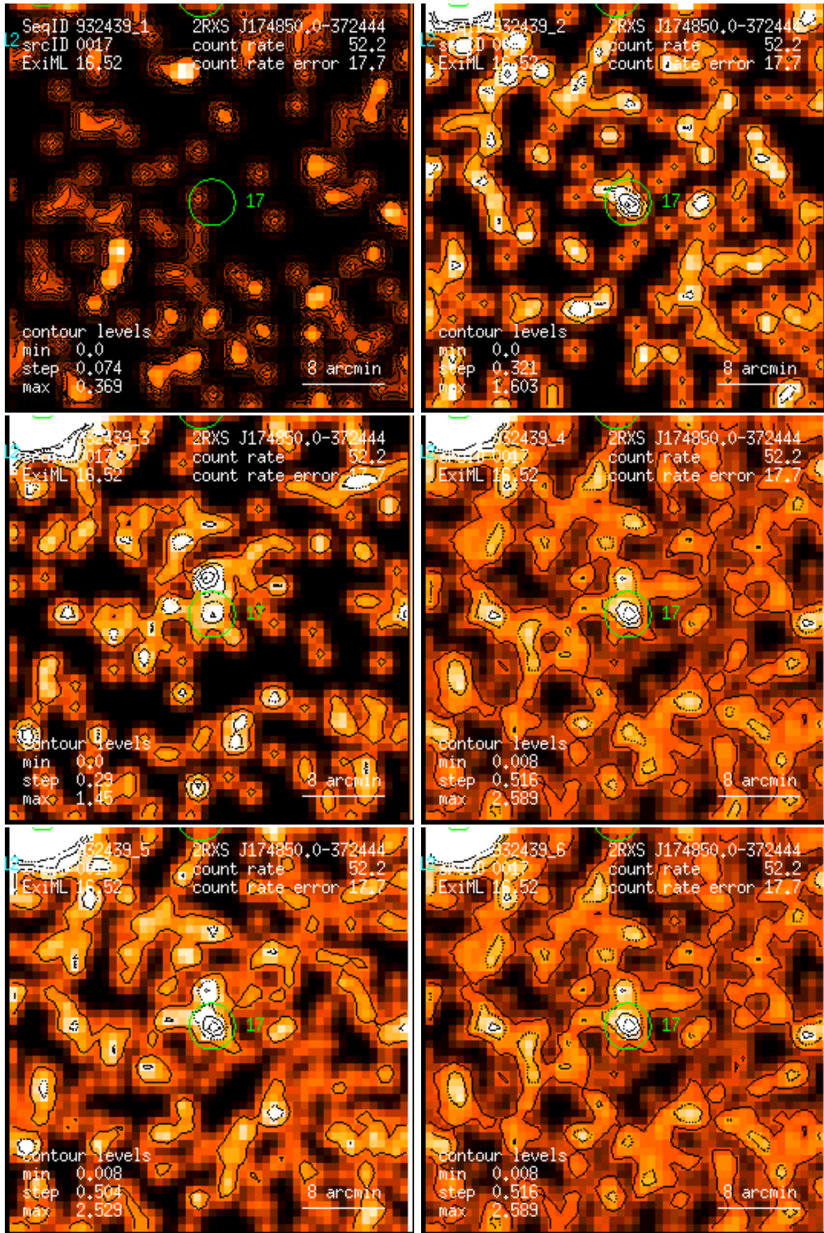
Figure 17: RASS 932439: detection 0017: band rate images, Gaussian filter: (1) PSPC channels 11 – 41, (2) 52 – 90, (3) 91 – 201, (4) 11 – 235, (5) 52 – 201, (6) 11 – 201. Broad band rates in counts/ks. Band rate contour levels in counts/ks/arcmin 2 .
