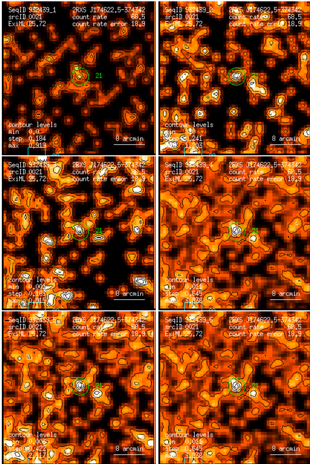
Figure 21: RASS 932439: detection 0021: band rate images, Gaussian filter: (1) PSPC channels 11 – 41, (2) 52 – 90, (3) 91 – 201, (4) 11 – 235, (5) 52 – 201, (6) 11 – 201. Broad band rates in counts/ks. Band rate contour levels in counts/ks/arcmin 2 .
