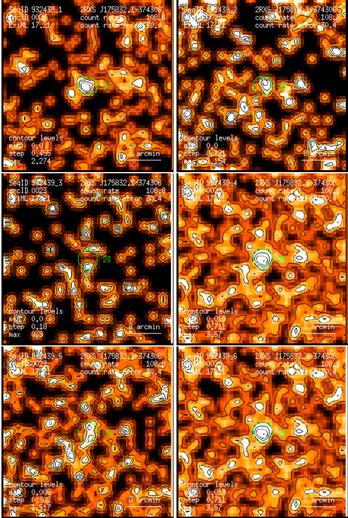
Figure 23: RASS 932439: detection 0023: band rate images, Gaussian filter: (1) PSPC channels 11 – 41, (2) 52 – 90, (3) 91 – 201, (4) 11 – 235, (5) 52 – 201, (6) 11 – 201. Broad band rates in counts/ks. Band rate contour levels in counts/ks/arcmin 2 .
