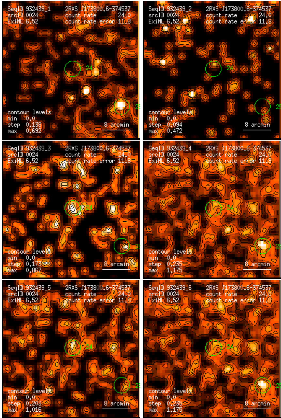
Figure 24: RASS 932439: detection 0024: band rate images, Gaussian filter: (1) PSPC channels 11 – 41, (2) 52 – 90, (3) 91 – 201, (4) 11 – 235, (5) 52 – 201, (6) 11 – 201. Broad band rates in counts/ks. Band rate contour levels in counts/ks/arcmin 2 .
