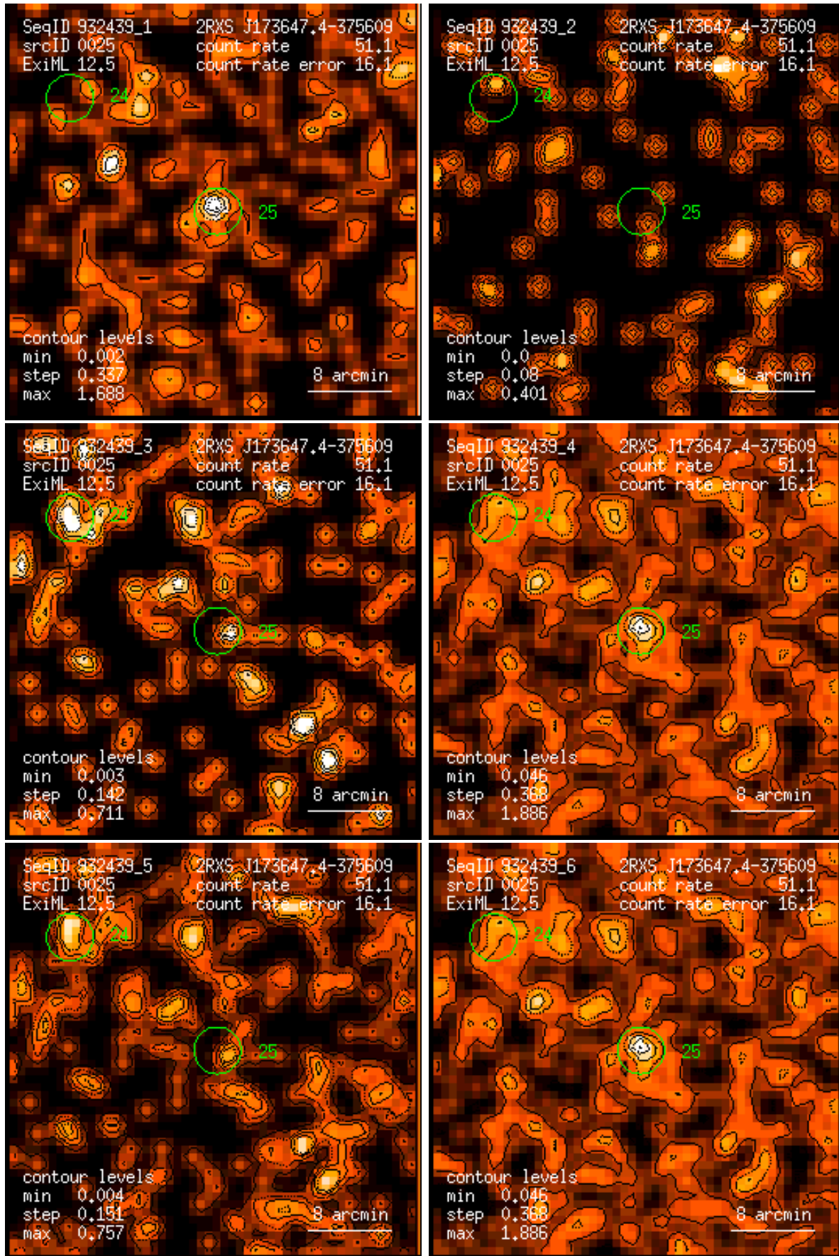
Figure 25: RASS 932439: detection 0025: band rate images, Gaussian filter: (1) PSPC channels 11 – 41, (2) 52 – 90, (3) 91 – 201, (4) 11 – 235, (5) 52 – 201, (6) 11 – 201. Broad band rates in counts/ks. Band rate contour levels in counts/ks/arcmin 2 .
