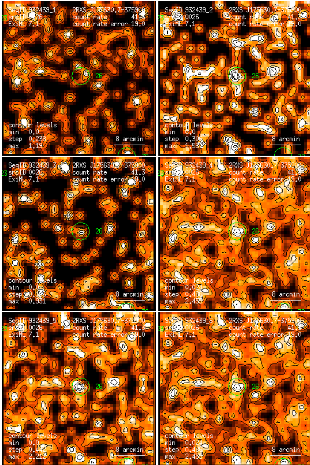
Figure 26: RASS 932439: detection 0026: band rate images, Gaussian filter: (1) PSPC channels 11 – 41, (2) 52 – 90, (3) 91 – 201, (4) 11 – 235, (5) 52 – 201, (6) 11 – 201. Broad band rates in counts/ks. Band rate contour levels in counts/ks/arcmin 2 .
